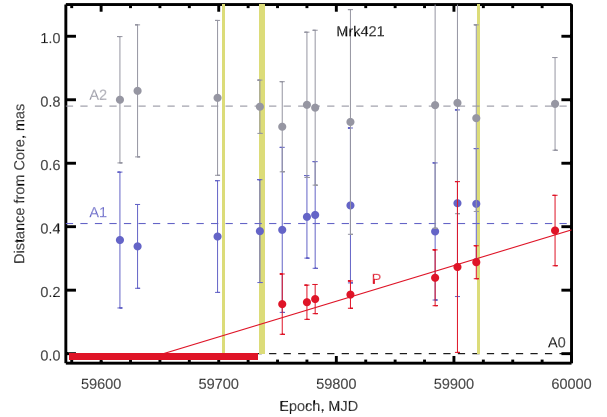
Fig. A.3. Distance from the core of jet components A1 (blue circles), A2 (gray circles), and P (red circles) versus time. The black dotted line indicates the position of the core, A0, the red line approximates the motion of knot P with the uncertainty of its ejection time shown by the red area at the bottom left, and yellow areas mark epochs of IXPE observations.
