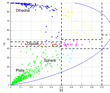
Figure 5: Polarization behavior of site 2. The buried objects are classified correctly in the expected regions.
