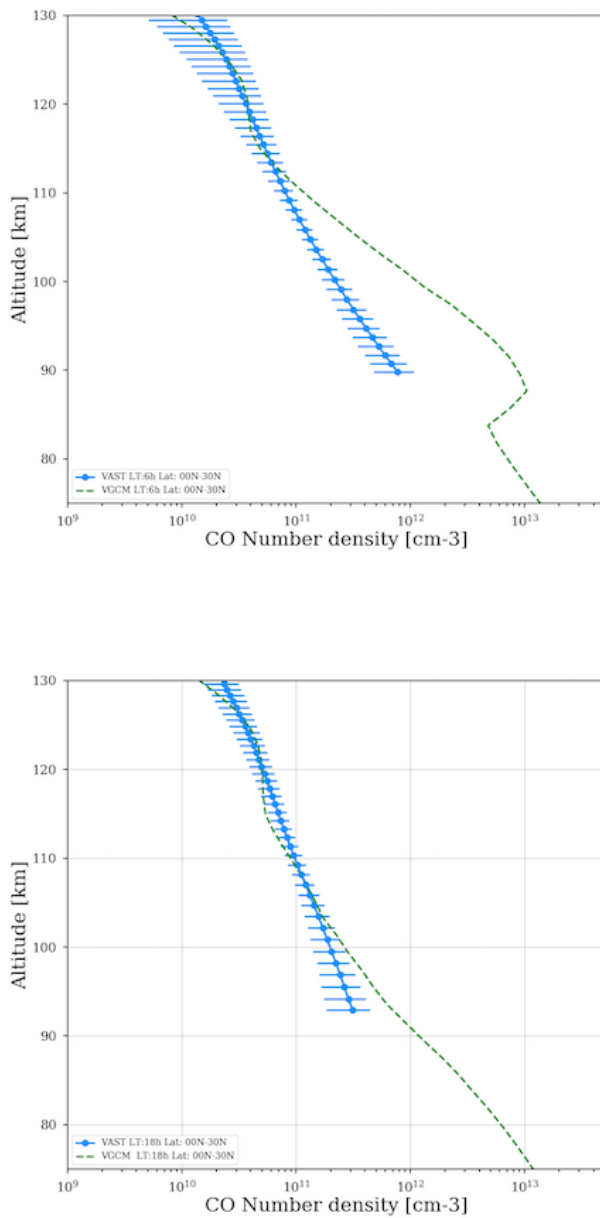
Figure 1: Example of comparison of simulated CO densities by the IPSL-VGCM (green dashed line) with retrieved measurements (blue dots) and standard deviations at equatorial latitudes (0-30N), extracted from the Venus Atmosphere from SOIR measurements at the terminator (VAST) (Vandaele et al.2016). Top: Morning terminator. Bottom: Evening terminator.
