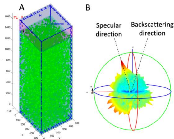
Figure 2: A: Subsurface model where 30% of the snow layer is occupied by randomly distributed 1-cm radius vacuum inclusions. B: Radiation pattern of the model shown in A for an incident plane wave arriving with an incidence angle of 20°. The signal returned in the backscattering direction is very small.
