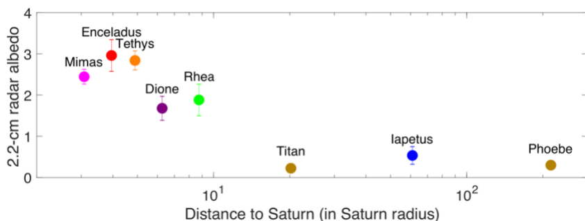
Figure 1: Averaged 2.2-cm disk-integrated radar albedos of Saturn's major satellites. The error bars show the dispersion of the dataset for each satellite.
