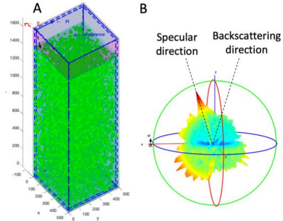
Figure 2: A: Subsurface model where 30% of the snow layer is occupied by randomly distributed 1-cm radius vacuum inclusions. B: Radiation pattern of the model shown in A for an incident plane wave arriving with an incidence angle of 20^\circ . The signal returned in the backscattering direction is very small.
