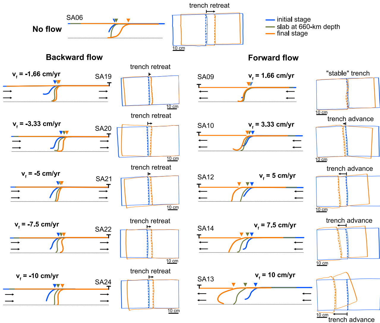
Figure 4. Slab geometry and horizontal position of the plates when subduction is initiated (blue), when the slab arrives at the 660-km discontinuity (green), and after \sim 50 Myr of subduction (orange), interpreted from lateral (left) and top (right) views of the 11 models. Stage 1 corresponds to the evolution of subduction from initiation (blue) to when the slab reaches the 660-km discontinuity (green), while stage 2 encompasses the subsequent time until the end of the experiment (orange). Initial model SA06 is reported on top, while other models, with a fixed plate and with backward mantle flow (left half of the figure) or forward mantle flow (right half of the figure), are reported below. The down-pointed triangles on lateral views represent the trench position at different experimental times, and pin-points indicate when a plate is fixed.
