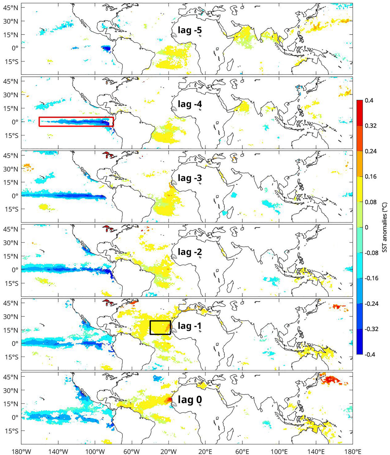
Figure 4. Identical to Figure 3 but for PC1CRU Senegal.
