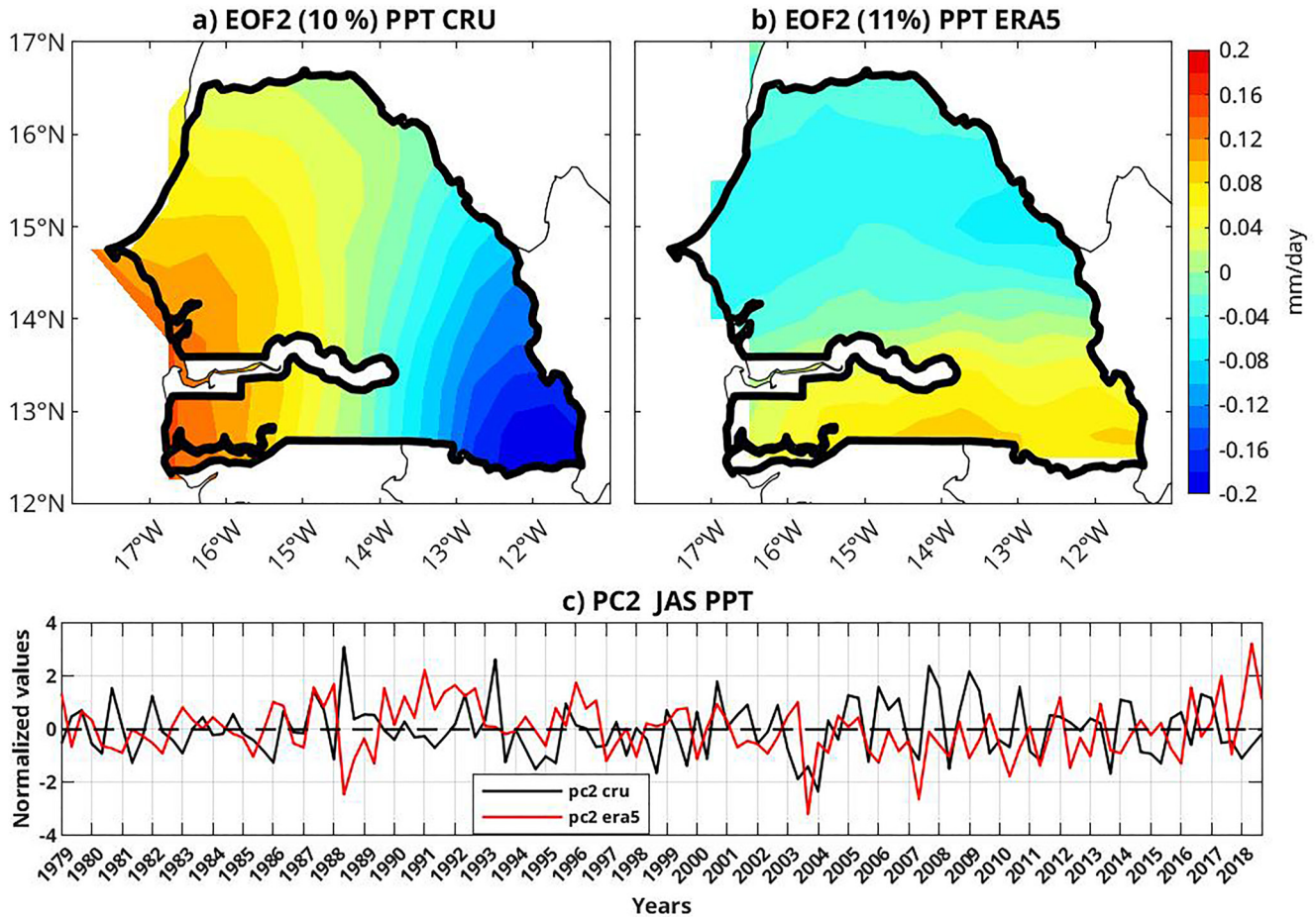
Figure A1. July, August, and September 1979–2018 EOF2 of precipitation (mm/day): (a) Climatic Research Unit (CRU) observations, (b) ERA5 reanalyzes, and (c) corresponding time series (black for CRU and red for ERA5).
