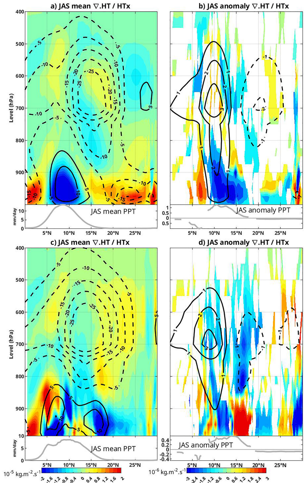
Figure 8. July, August, and September 1978–2018 ERA5 reanalyses, average (left) and linear regressions on the PC1CRU index (right) in vertical meridional sections over the ocean (22°W–17°W, (a, b)) and over the continent (10°–5°W, (c, d)): Divergence of moisture transport (colors) and zonal moisture transport (black contours, solid for positive, dashed for negative), superimposed on precipitation (gray line in panels at the bottom). Only values significant at the 95% confidence level are plotted.
