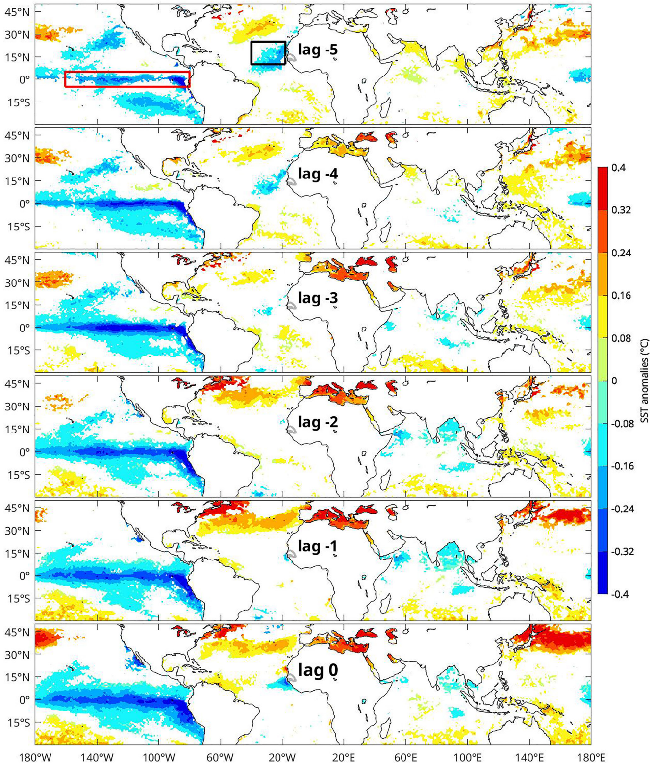
Figure 3. Linear regression of Sea Surface Temperature (SST) anomalies on PC1CRU Sahel (°C) from lags -5 to 0 (indicating that SST precedes PC1CRU Sahel by 5 to 0 months). Only values significant at the 95% confidence level are plotted. The red box outlines the eastern equatorial Pacific ( 180^{\circ}\text{W} – 80^{\circ}\text{W} , 5^{\circ}\text{S} – 5^{\circ}\text{N} ). The black box frames the Northeastern Tropical Atlantic ( 40^{\circ}\text{W} – 17^{\circ}\text{W} , 10^{\circ}\text{N} – 25^{\circ}\text{N} ).
