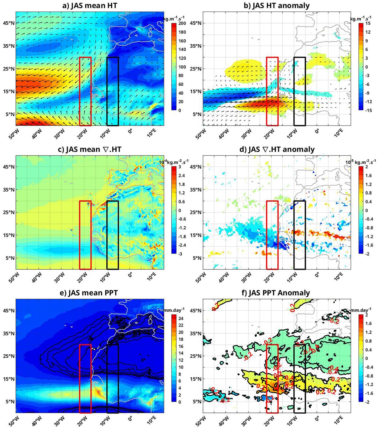
Figure 7. July, August, and September 1978–2018 ERA5 reanalyses, average (left) and linear regression on PC1CRU index (right): (a, b) magnitude (colors) and direction (arrow) of moisture transport (HT). (c, d) Divergence of moisture transport ( \nabla \cdot HT ). (e, f). Precipitation (PPT). In panel (e), values less than 1 mm/day are outlined in black (intervals of 0.1 mm/d). In panels (b), (d), and (f), only values significant at the 95% confidence level are plotted. In panel (f), correlations are depicted using black contours with intervals of 0.2. Red and black frames indicate the location of the meridional-vertical sections plotted in Figures 8 and 9.
