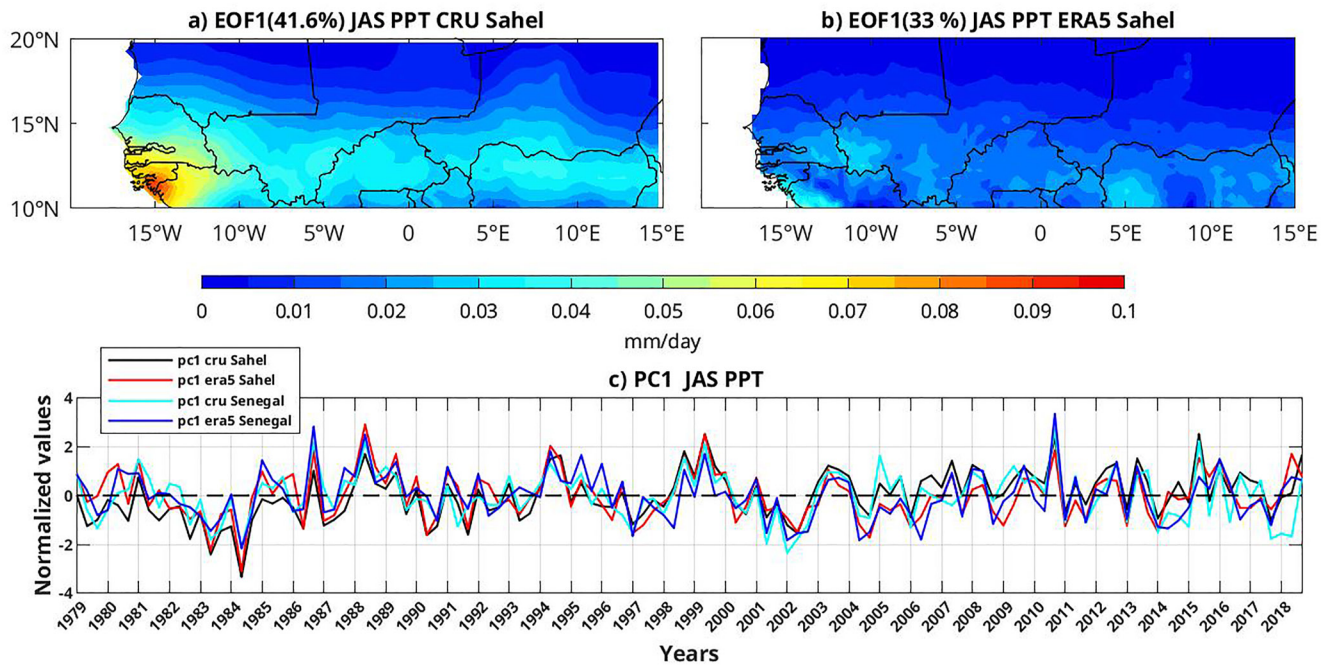
Figure A3. July, August, and September 1979–2018 precipitation, EOF1 over the Sahel (mm/day): (a) in Climatic Research Unit (CRU) observations, (b) in ERA5 reanalyses and (c) their corresponding time series (CRU in black and ERA5 in red). CRU Senegal (cyan) and ERA5 Senegal (blue) time series are also plotted.
