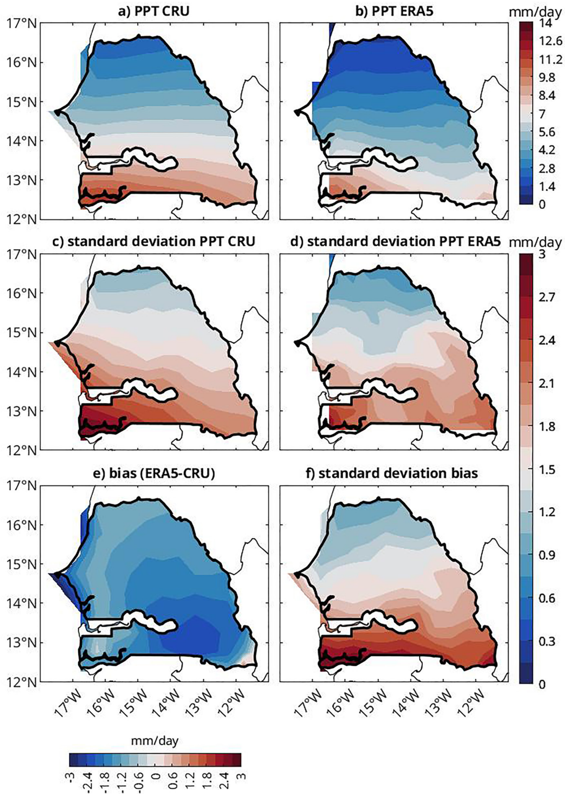
Figure 1. July, August, and September 1979–2018 precipitation (PPT) in Senegal (mm/day): (a) Climatic Research Unit (CRU) observations, (b) ERA5 reanalyses, (c) Standard deviation of CRU anomalies, (d) Standard deviation of ERA5 anomalies, (e) mean bias between CRU observations and ERA5 reanalyses, (f) Standard deviation of the bias.
