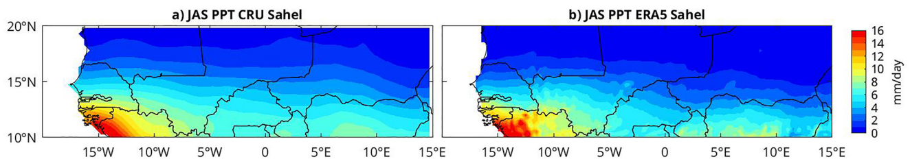
Figure A2. July, August, and September 1978–2018 Climatic Research Unit (left) and ERA5 (right) precipitation.
