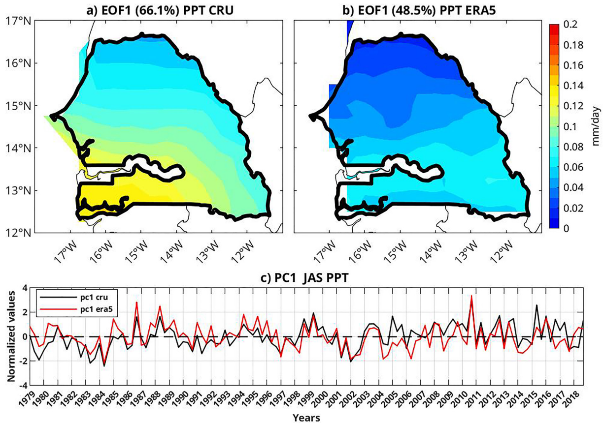
Figure 2. July, August, and September 1979–2018, principal mode of variability (EOF1) for precipitation (PPT) anomalies (mm/day): (a) Climatic Research Unit (CRU) observations, (b) ERA5 reanalyses and (c) corresponding time series (black contours for CRU, red contours for ERA5).
