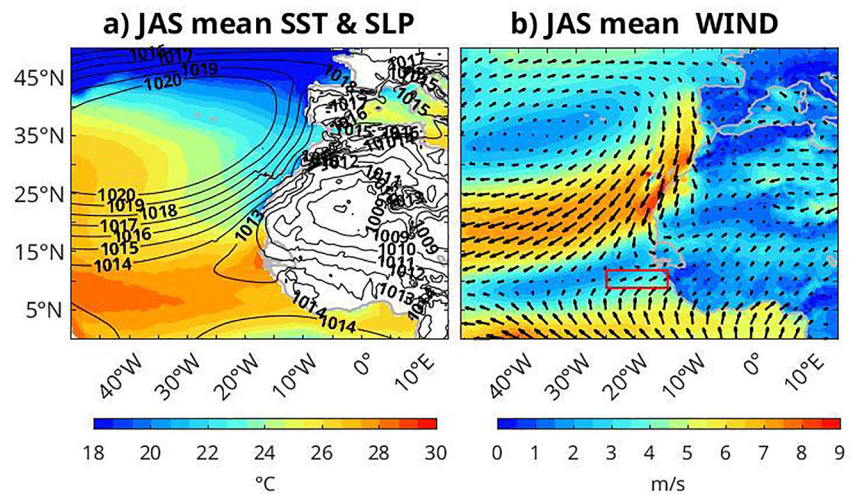
Figure 5. July, August, and September 1979–2018 ERA5 reanalyses: (a) Sea Surface Temperature (colors) and Sea Level Pressure (black contours). (b) 10-m wind speed (colors) and direction (arrows). The red frame indicates the location of the West African Westerly Jet (25°W–14°W, 9°N–12°N).
