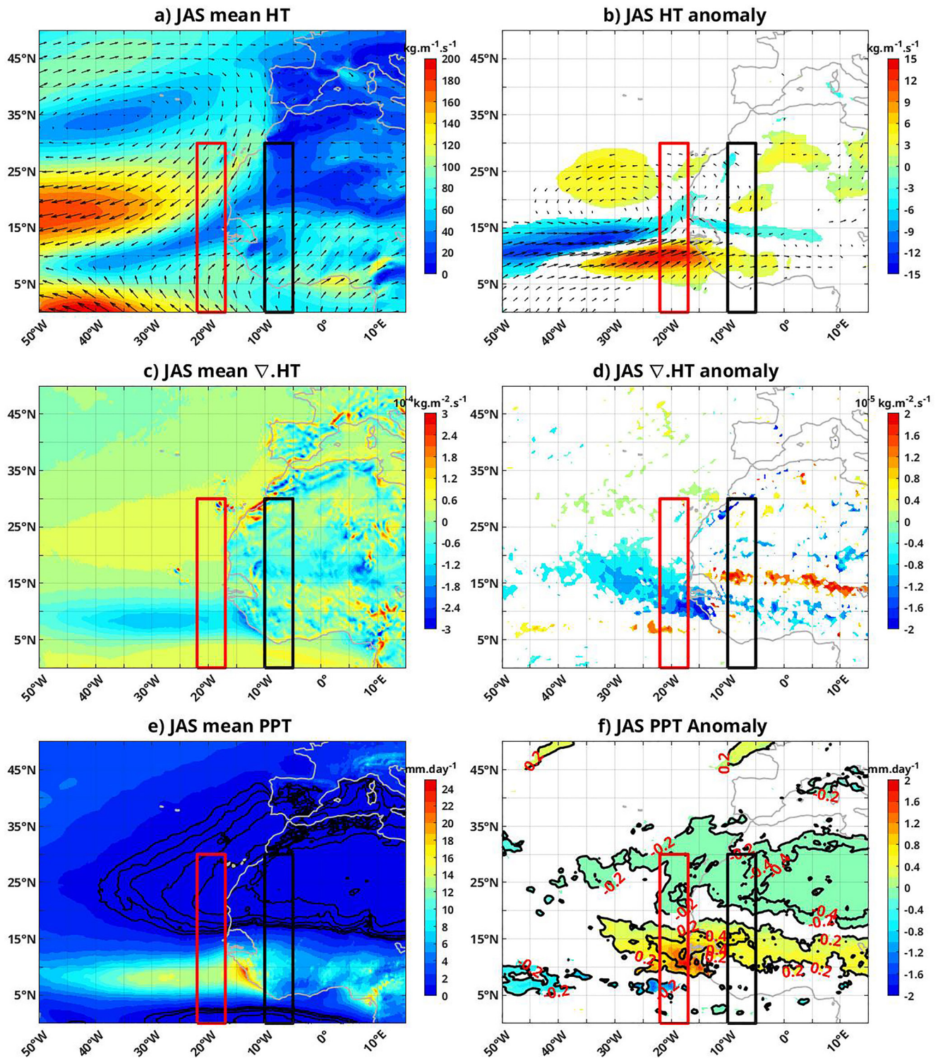
Figure 7. July, August, and September 1978–2018 ERA5 reanalyzes, average (left) and linear regression on PC1CRU index (right): (a, b) magnitude (colors) and direction (arrow) of moisture transport (HT). (c, d) Divergence of moisture transport ( \nabla\cdot\text{HT} ). (e, f). Precipitation (PPT). In panel (e), values less than 1 mm/day are outlined in black (intervals of 0.1 mm/d). In panels (b), (d), and (f), only values significant at the 95% confidence level are plotted. In panel (f), correlations are depicted using black contours with intervals of 0.2. Red and black frames indicate the location of the meridional-vertical sections plotted in Figures 8 and 9.
