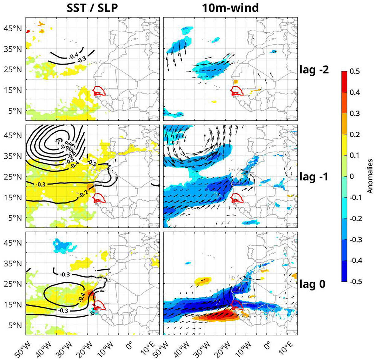
Figure 6. Linear regression of ERA5 reanalyses on PC1CRU, from lags -2 (ERA5 leads PC1CRU by 2 months) to lag 0. Left: Sea Surface Temperature (colors, ^{\circ}\text{C} ) and Sea Level Pressure (black contours, hPa). Right: 10m-wind speed (colors, m/s) and direction (arrow). Only values significant at the 95% level are plotted.
