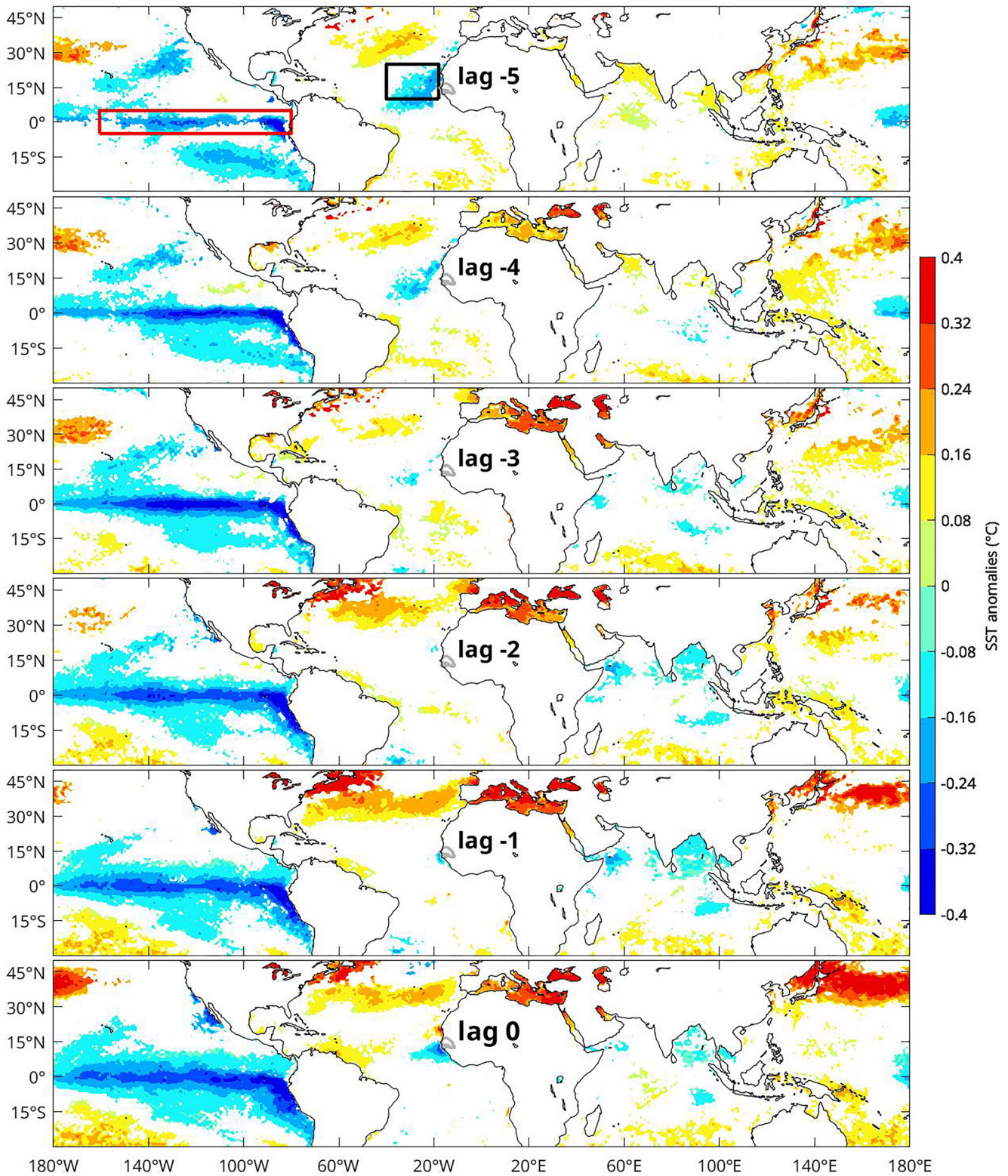
Figure 3. Linear regression of Sea Surface Temperature (SST) anomalies on PCICRU Sahel ( ^{\circ}\text{C} ) from lags -5 to 0 (indicating that SST precedes PCICRU Sahel by 5 to 0 months). Only values significant at the 95% confidence level are plotted. The red box outlines the eastern equatorial Pacific ( 180^{\circ}\text{W} – 80^{\circ}\text{W} , 5^{\circ}\text{S} – 5^{\circ}\text{N} ). The black box frames the Northeastern Tropical Atlantic ( 40^{\circ}\text{W} – 17^{\circ}\text{W} , 10^{\circ}\text{N} – 25^{\circ}\text{N} ).
