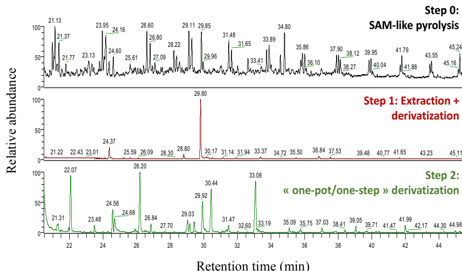
Figure 2: Comparison of the chromatograms obtained after the analysis of the OM2 sample in three steps: SAM-like pyrolysis: Step 0, solid-liquid extraction + MTBSTFA derivatization: step 1, “one-pot/one-step” extraction + derivatization (step 2).
