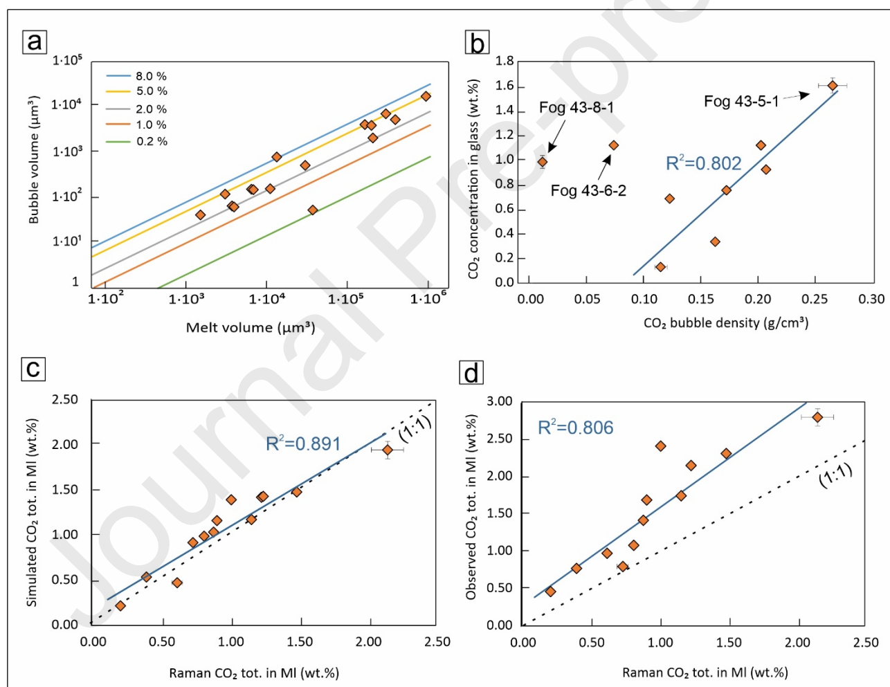
Figure 8. (a) Plot of bubble volumes as a function of MI volumes; isovolumetric lines corresponding to bubble/MI volume ratios of 0.2 %, 1.0 %, 2.0 %, 5.0 %, and 8.0 % are also shown. (b) The plot shows a positive correlation between the CO 2 calculated in the glass and the density of the shrinkage bubble, except for the two samples (Fog 43-8-1 and 43-6-2) which exhibit intense Raman peaks associated with carbonates, specifically Fe-magnesite and nahcolite crystals on the bubble wall (Fig. 2). As shown in (b), the overlooked presence of carbonates in the bubble leads to an underestimation of the total CO 2 content. Excluding these two outliers, the samples show a good
