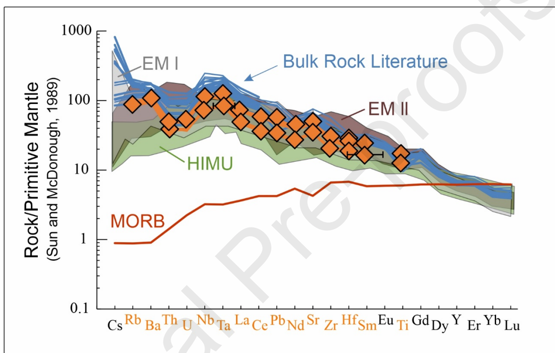
Figure 5. Primitive mantle-normalised (Sun and McDonough, 1989) trace element patterns in MI samples (orange patterns; average values from all samples are used). The trace element patterns are intermediate between the compositional ranges of enriched mantle sources (EM-I and EM-II; data from Willbold and Stracke, 2006) and the HIMU mantle source (Willbold and Stracke, 2006). Note the significant Nb and Ta enrichment relative to the light REE. The red line identifies the compositions of Mid-Oceanic Ridge Basalts (MORB; Sun and McDonough, 1989).
