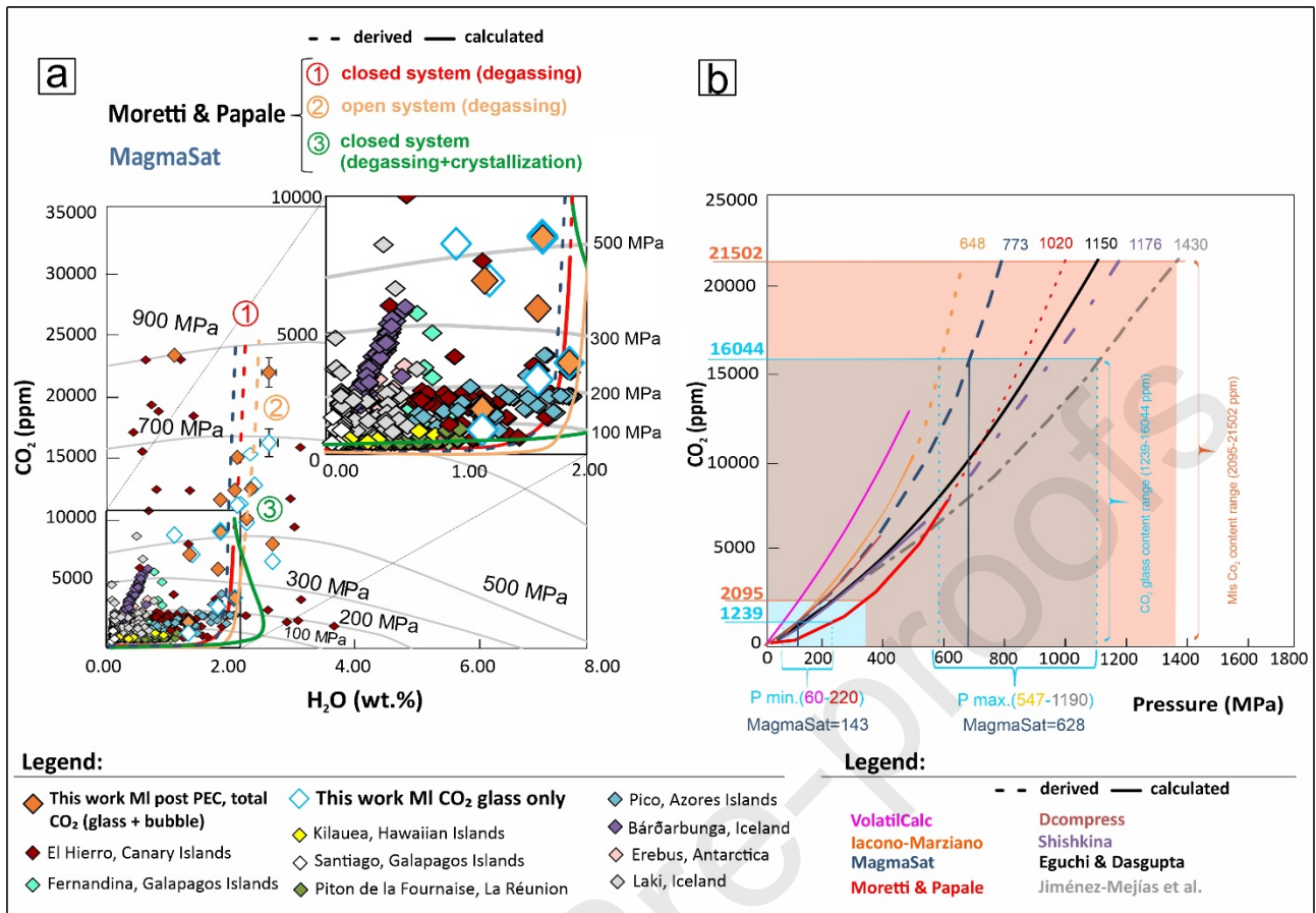
Figure 9. (a) \text{H}_2\text{O} and \text{CO}_2 concentration in studied MI and in other OIB occurrences. Isobars were calculated using an average composition of our MI samples at temperature of 1150\text{ }^\circ\text{C} and an oxygen fugacity of \Delta\text{FMQ} + 1.5 (Moussallam et al., 2019). Degassing paths, in a closed system, were calculated using the volatile saturation models by Moretti et al. (2003) and MagmaSat (Ghiorso and Gualda, 2015), with the same input melt composition and temperature and volatile contents of 21502 ppm and 2.0 wt.% for \text{CO}_2 and \text{H}_2\text{O} respectively. (b) In the \text{CO}_2 content vs. Pressure graph, different saturation models are compared. The solid lines represent the outputs of the different models, instead the dashed lines represent the extrapolations of these models.
