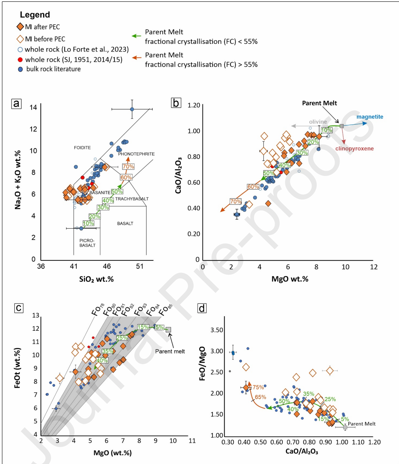
Figure 4 Total alkali-silica diagram (a) and major element compositions of melt inclusions (b, c, d) together with whole-rock compositions from Hildner et al. (2011, 2012), Lo Forte et al. (2023) and Mata et al. (2017). The solid lines are liquid lines of descent (LLD), calculated from a primitive parent melt (SiO 2 42.14 wt.%, MgO 9.79 wt.%, FeO 12.03 wt.%, Al 2 O 3 12.41 wt.%, CaO 12.96 wt.%) using Petrolog3 (Danyushevsky and Plechov, 2011). The LLD are calculated assuming initial H 2 O content of 2 wt.% and oxygen fugacity of \Delta\text{FMQ} + 1.5 (Moussallam et al., 2019). We used the melt-mineral equilibrium models of Danyushevsky (2001) for olivine, clinopyroxene and plagioclase, and of Ariskin and Barmina (1999) for magnetite. The orange LLD was calculated for FC > 55%, to fit the more evolved MI (d). The grey area represents the range of forsterite component (Fo 80-85 ) in the analysed olivines hosting MI (a).
