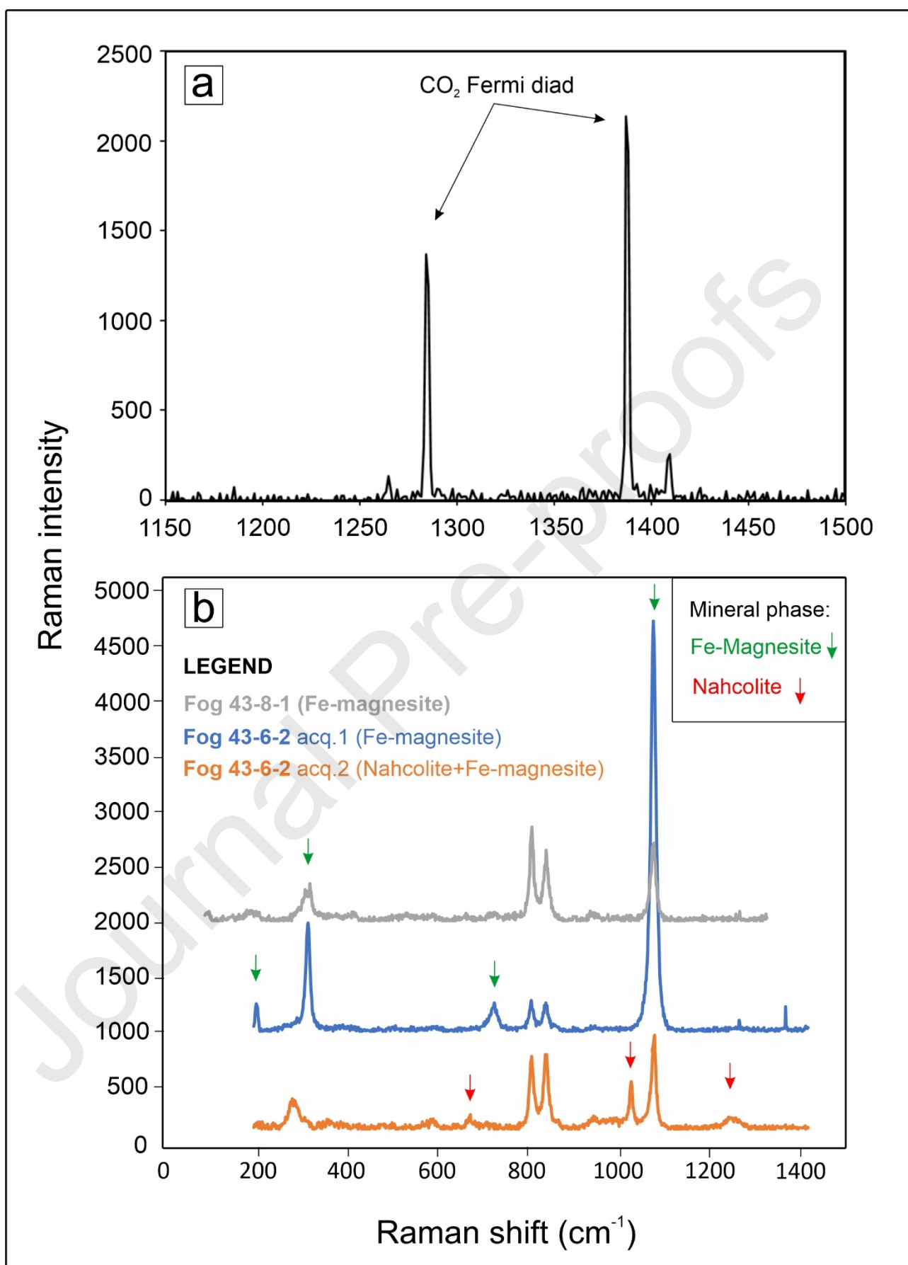
Figure 2. (a) Raman spectrum of melt inclusion shrinkage bubble (sample Fog 43-8-1). The bubble is made of pure CO 2 , as revealed by the two strong peaks at 1284 and 1387 cm -1 , identified as Fermi
