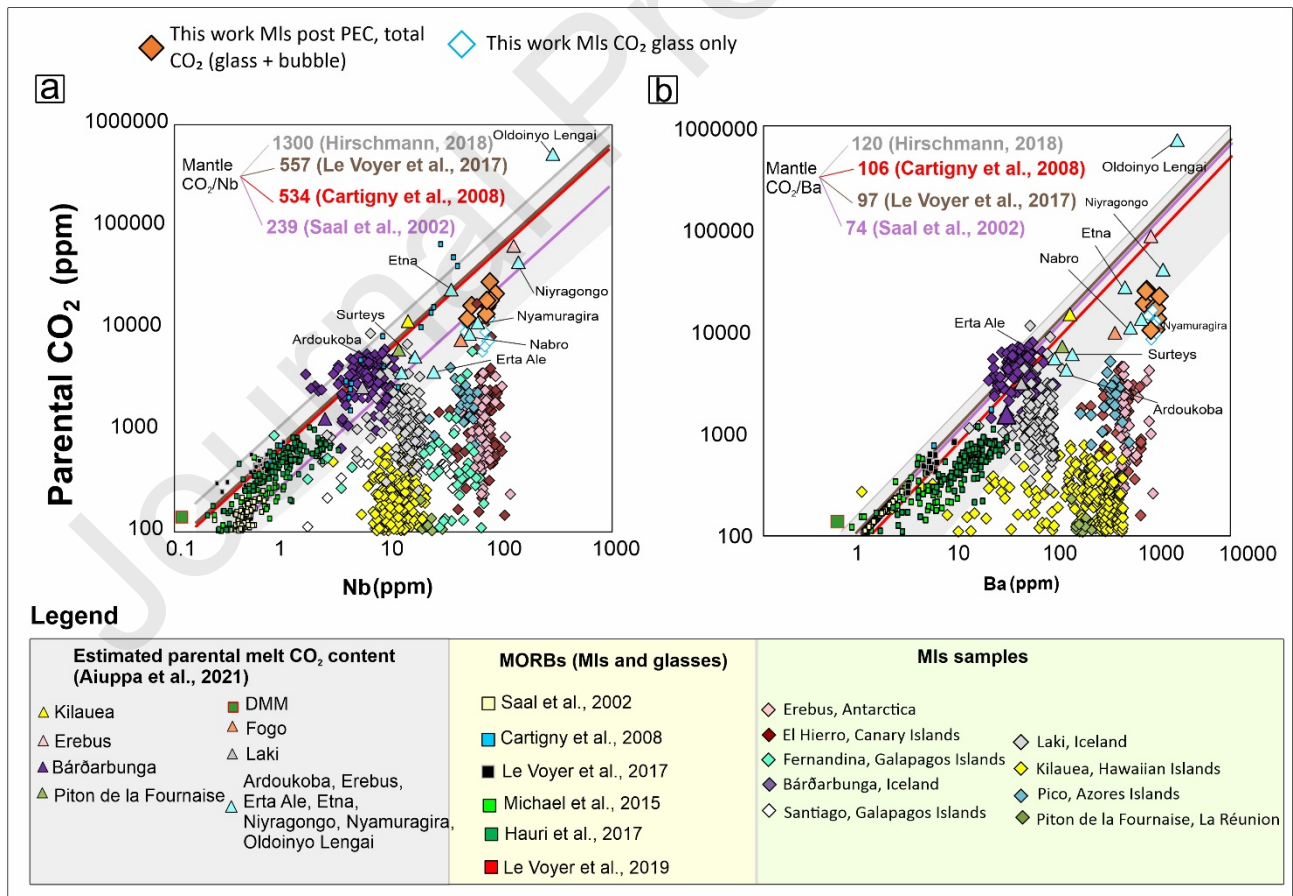
Figure 10. CO 2 /trace element ratios. (a) In the Nb versus CO 2 plot, most of the literature “degassed” MI and our MI with the CO 2 content measured in the glass only (white diamond with
