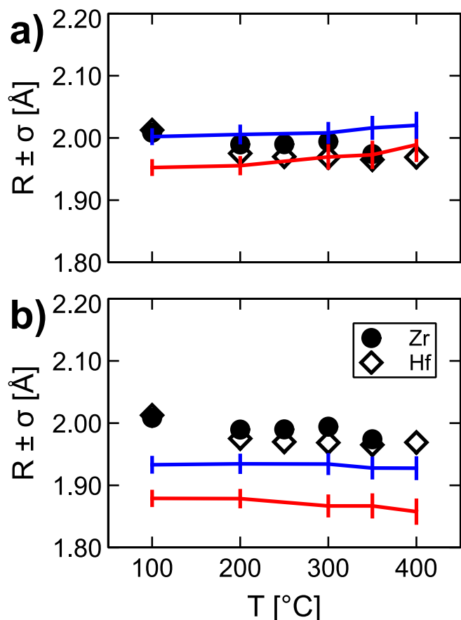
Fig. 7. a) Mean distances of the 6F or O atoms closest to the central cation, weighted with R^{-2} for two sets of Lennard-Jones parameters: \sigma = 1.8 Å, \varepsilon = 20.92 kJ/mol (blue); \sigma = 3.6 Å, \varepsilon = 4.184 \cdot 10^{-3} kJ/mol (red). Experimental EXAFS results for Zr and Hf (symbols) shown for comparison. b) Same for the 4 closest F and O atoms. (For interpretation of the references to colour in this figure legend, the reader is referred to the web version of this article.)
