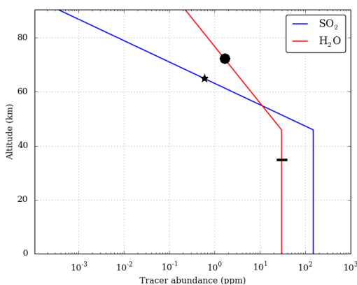
Figure 2: Vertical profile of the tracer abundance relaxation profile. The black represents the value for the deep atmosphere [4], the star is
