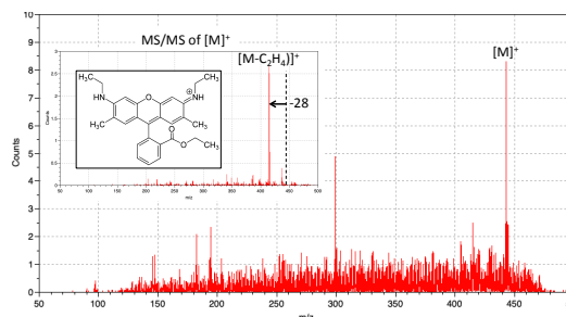
Figure 3 : MS detection and (inset) MS/MS analysis of Rhodamine 6G at 50 fmol/mm 2 with LDI-MS.
