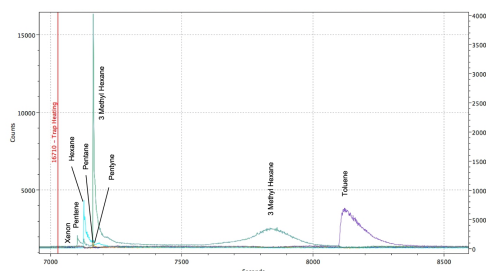
Figure 2 : chromatogram obtained with the MXT5 column of the flight model tested at NASA/GSFC for the analysis of a mixture of hydrocarbons.
