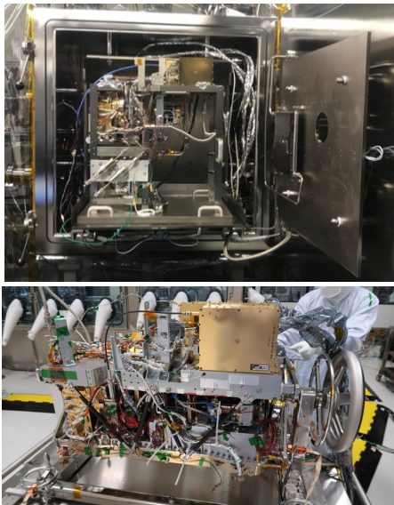
Figure 1 : MOMA flight model in the thermal chamber at NASA/GSFC (upper picture) and integrated in its final configuration with the rest of the ALD at TAS-I (lower picture)
