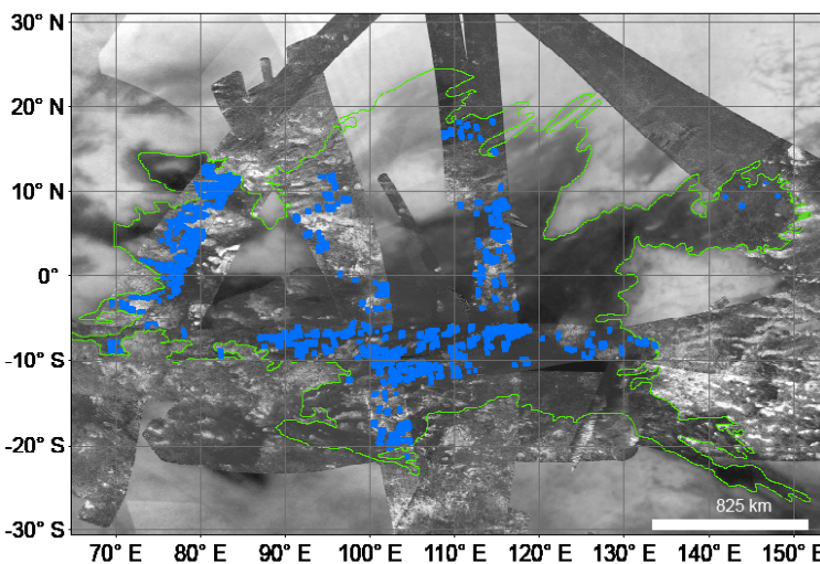
Fig. 1 Width and spacing measurements in the Belet Sand Sea. The estimated maximum extent is in green and the locations of the dune width and spacing measurements are in blue.
