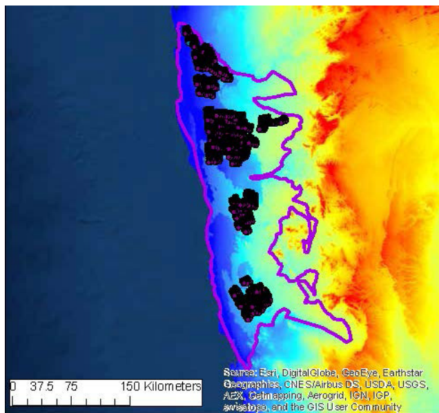
Fig. 2 Dune width and spacing measurements in the Namib Sand Sea of southwest Africa. The sand sea margin is in purple. The points represent measurement sites. SRTM elevation data is represented by the colored heat map.
