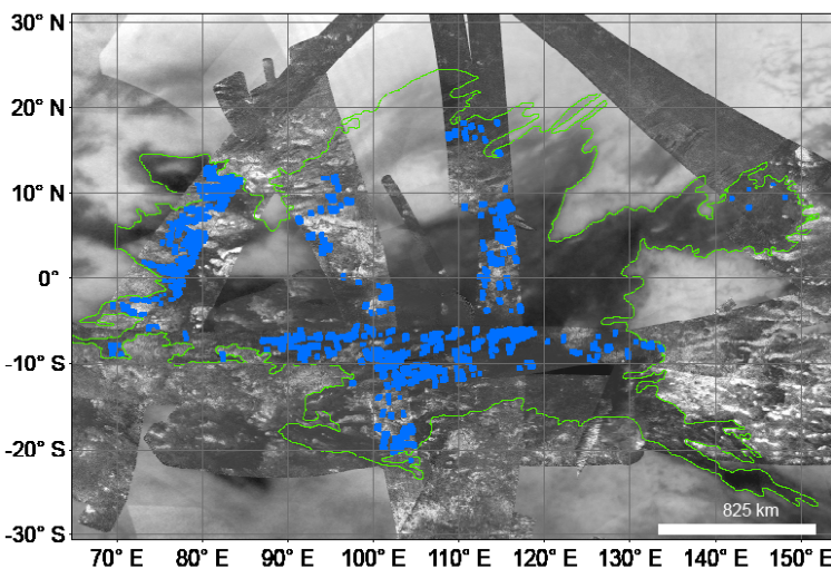
Fig. 1 Width and spacing measurements in the Belet Sand Sea. The estimated maximum extent is in green and the locations of the dune width and spacing measurements are in blue.
