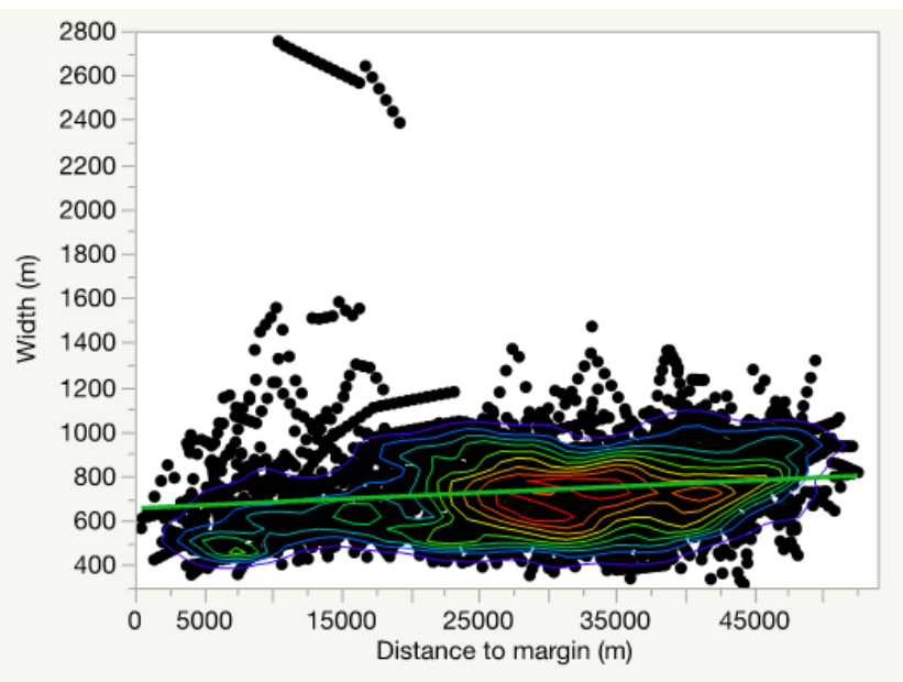
Fig. 3 Dune width according to distance from the sand sea margin in the Namib Sand Sea. The colored rings are 10% quantiles. The best fit line has an r^2 value of 0.023674 and a p -value of 0.005.
