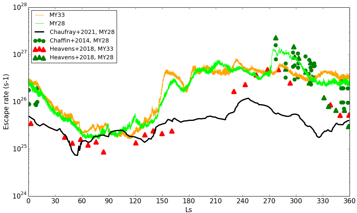
Figure 1. H escape rate simulated for MY28 (light green line) and MY33 (orange line). The black thin line shows the escape rate for MY28 simulated with the previous model version, taken from Chaufray et al. (2021). The green and red symbols represent measured values of the H escape rate during MY28 and MY33, respectively, taken from Chaffin et al. (2014) and Heavens et al. (2018)
