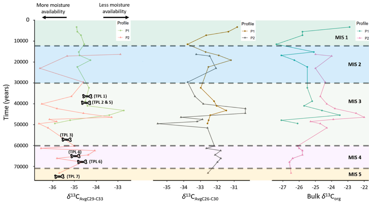
Fig. 3. The weighted average of the three dominant n -alkanes ( \delta^{13}\text{C}_{\text{AvgC29-C33}} ) n -alkanoles ( \delta^{13}\text{C}_{\text{AvgC26-C30}} ) and bulk \delta^{13}\text{C}_{\text{org}} plotted against time (years). Bones plotted on \delta^{13}\text{C}_{\text{AvgC29-C33}} represent H. sapiens fossils from TPL. Fossils have not been directly dated and are presented at approximate ages based on the interpolated ages from the sediment profiles they were recovered from.
