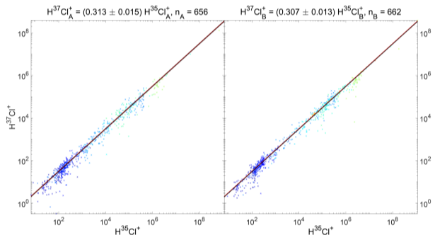
Figure 3. \text{H}^{37}\text{Cl}^+ as a function of \text{H}^{35}\text{Cl}^+ for \text{H}^{35}\text{Cl}^+/\text{H}^{37}\text{Cl}^+ > 0.7 , weighted average and uncertainties (resp. solid and dotted black lines). Data are color-coded for time between 08/01/2014 (blue) and 05/09/2016 (red). \text{H}^{37}\text{Cl}^+ was determined by subtracting ^{12}\text{C}^{32}\text{S}_2^{2+} from the sum signal at m/Z 38 and only values \text{H}^{37}\text{Cl}^+ > 0 are taken into account. ^{12}\text{C}^{32}\text{S}_2^{2+}/^{12}\text{C}^{32}\text{S}_2^+ values from figure A1.
