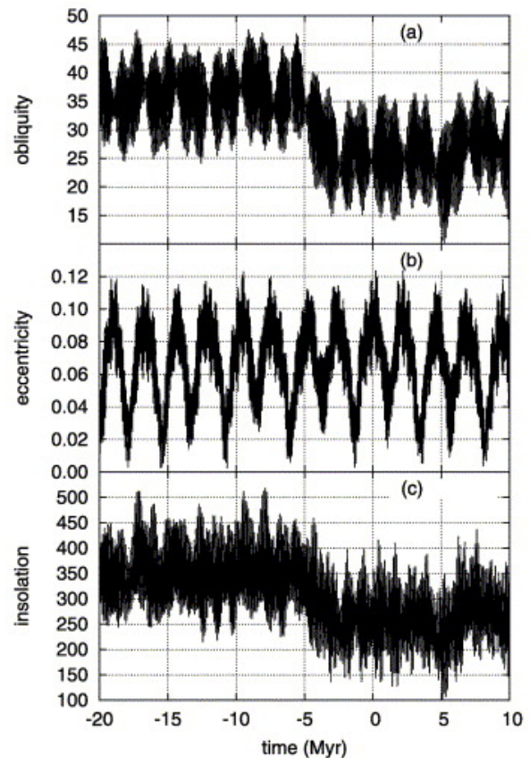
Figure 1: Evolution of the obliquity (a), eccentricity (b) and the north pole insolation (c) at the summer equinox ( L_s = 90^\circ ) from -20 to +10 million years, provided by Laskar et al. [2004] using the most recent data for the rotational state of Mars, and a new numerical integration of the Solar System)
