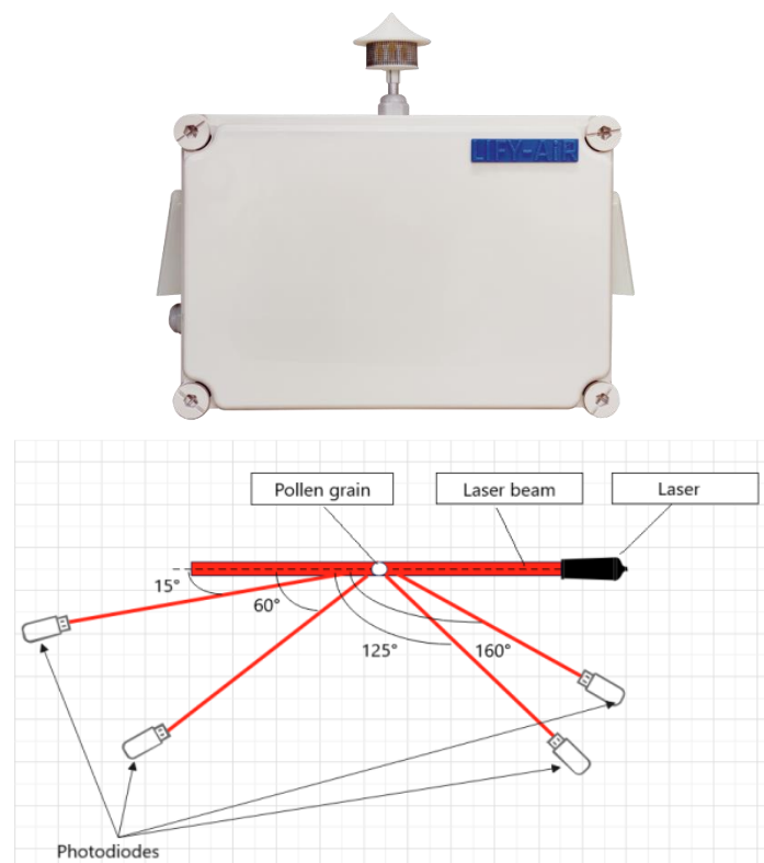
Figure 1. The Beenose sensor, with a picture of the instrument ( top panel ) and principle of measurement ( lower panel ).
