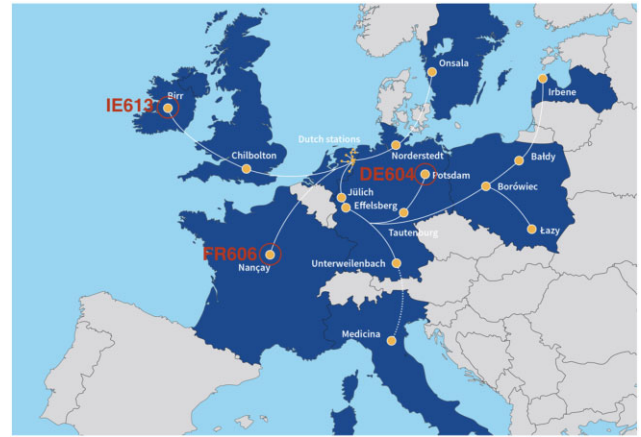
Figure 1. Map showing the location of LOFAR stations across Europe. 38 stations are located in the Netherlands, while 14 (soon 15) stations are located in seven (soon eight) other European countries. Here are highlighted the three stations that were used in the first case study described in Section 3: the Irish IE613, the French FR606, and the German DE604 stations.
