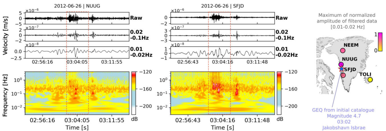
Figure A3. The catalogue event occurred on 2012-06-26 at 03:02 a.m. at Jakobshavn Isbrae, magnitude 4.7. Each subfigure shows the raw signal, the filtered signal in two frequency bands (0.02–0.1 and 0.01–0.02 Hz) and a spectrogram with signal intensity in decibels. Stations are shown on a map of Greenland, coloured according to the amplitude of the filtered signal in 0.01–0.02 Hz. The event is represented by a blue star. The signal from events is framed by red dotted lines.
