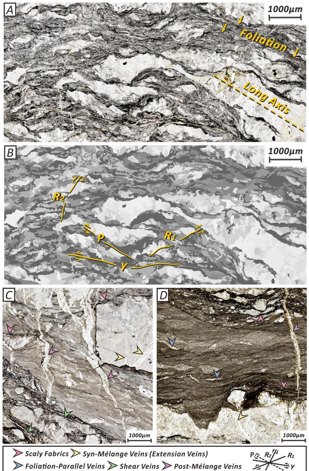
Figure 4. Photomicrographs of samples collected from (a) the Waterfall Bay mélangé, (c) Hyuga mélangé, and (d) Kure mélangé under plane-polarized light. (a) The foliation of the mudstone matrix is marked by yellow arrows. It is parallel to the long axes of sandstones (dashed yellow line). (b) Line drawing of the photomicrograph (a), where the Y-P-R surfaces along with the shear sense are annotated. (c, d) Pink arrows indicate the scaly fabrics characterized by dark seams due to pressure solution. Yellow, blue, green, and purple arrows mark the extension veins, foliation-parallel veins, shear veins, and the post-mélange veins, respectively.
