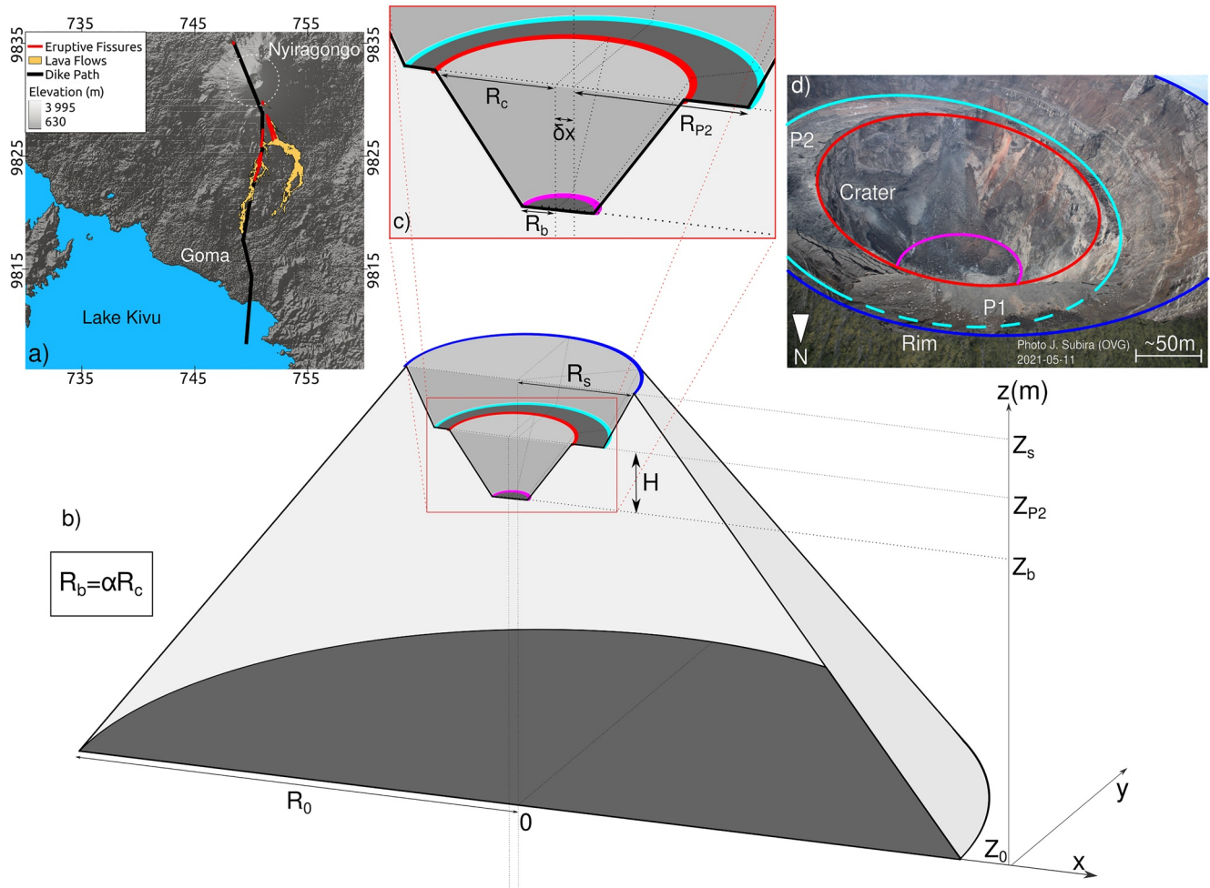
Figure 1. (a) Elevation map of Nyiragongo region also showing the May 2021 lava flow in orange and eruptive fissures in red as well as the trace of the dike modeled by Smittarello et al. (2022) in black. (b) Schematic of the simplified geometry of Nyiragongo topography. (c) Close up view of the collapsed crater. See parameter description in Table 2. (d) Nyiragongo crater seen from helicopter on the 5 November 2021. Credit J. Subira, Observatoire Volcanologique de Goma. P1 and P2 are the remnants of the platforms formed during the 1977 and 2002/2021 eruptions, respectively.
