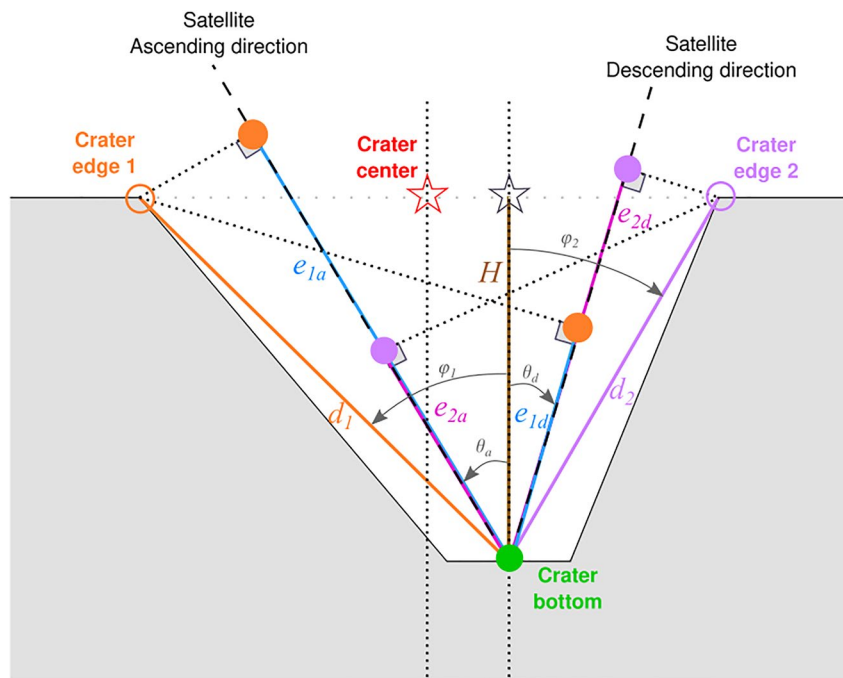
Figure 5. Using ascending and descending LOS to determine crater asymmetry along range direction.
