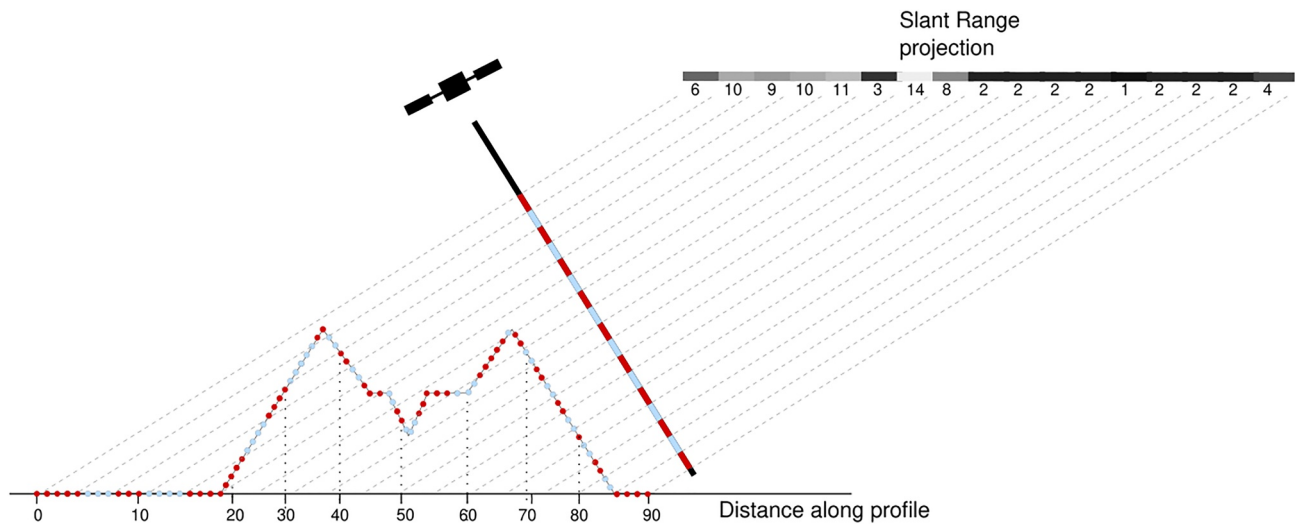
Figure 4. Simplified amplitude simulation methodology. Topographic profile is regularly sub-sampled and each point is projected on the slant range direction. For each interval in slant range, we sum all individual contributions to get the simplified simulated amplitude.
