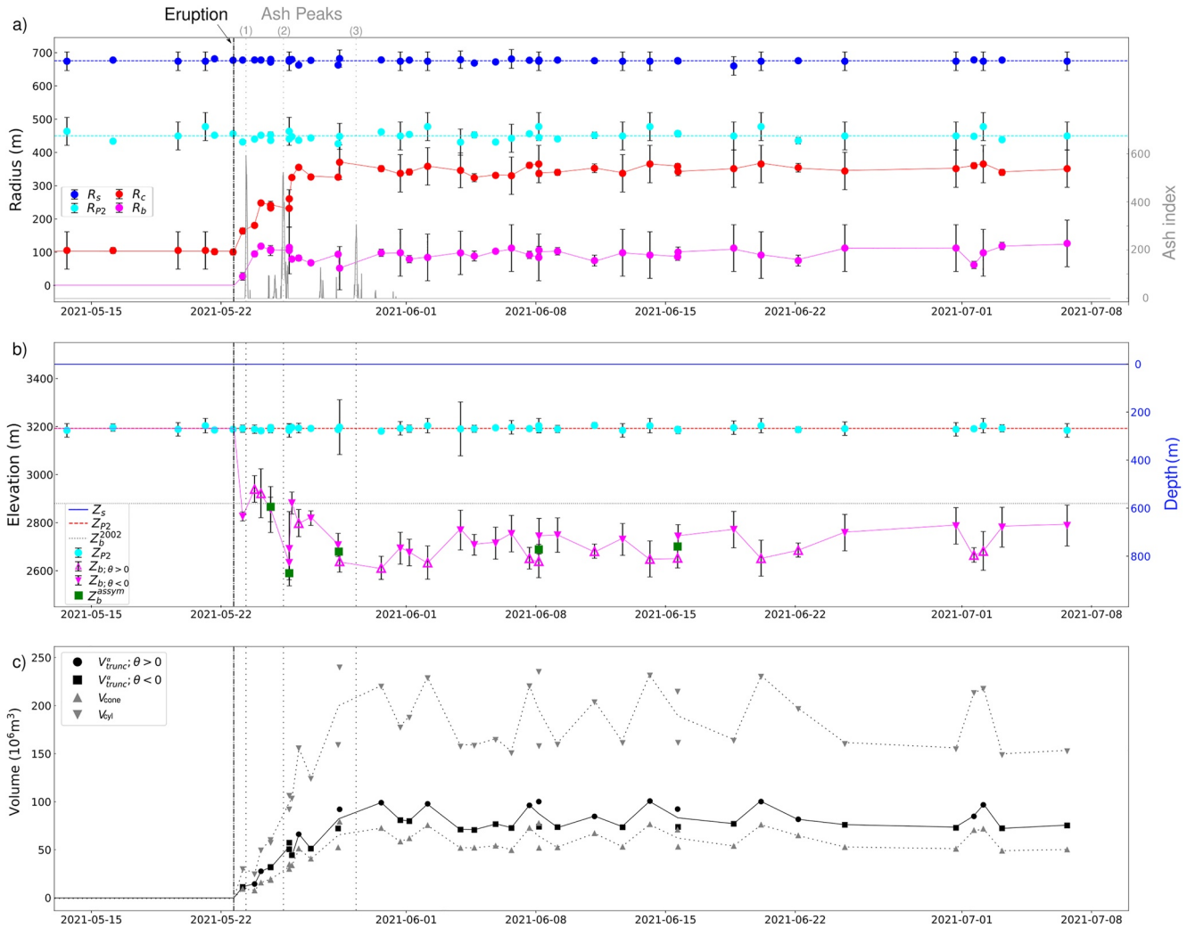
Figure 6. Time series of crater measures. Summit (dark blue), P2 (cyan), collapse crater (red) and bottom crater (magenta) radii (a) and elevation (b) time series obtained by manually picking four ellipses on each SAR image. Error bars in (a) represents 2, 3, 4, and 5 times the azimuth pixel spacing, respectively. Ash index computed using SEVIRI data spanning 13-05-2021 to 08-07-2021 from Smittarello et al. (2022) is shown in gray. Error bars in (b) on Z_{p2} represents 5 times the range pixel spacing. Error bars on Z_b are computed using Equation 7. In panel (b), green square mark values measured from both incidence angle, taking into account possible asymmetry of the crater. (c) Volume estimates derived from radius and elevation values for a truncated cone (black line). Square and dots are for measurements from negative and positive incidence angles, respectively. Minimum and maximum volume estimates corresponding to a cone (top gray triangles) and a cylinder (bottom gray cylinder), respectively, are also shown.
