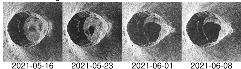
Figure 2. Subset of the CSK ascending images in radar geometry showing close view of the Nyiragongo crater from 2021 to 05-16 to 2021-06-08.
