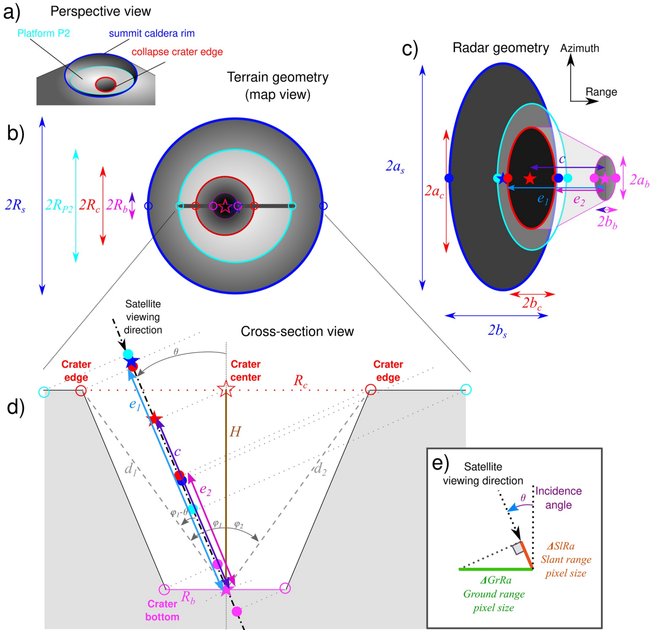
Figure 3. Methodology for estimating the collapsed crater radius and depth, assuming an idealized circular shape of the summit rim (blue), P2 platform (cyan), crater edge (red) and crater bottom (magenta). (a) Perspective view. (b) Map view. (c) Radar geometry view. (d) Cross section view. The incidence angle \theta is counted negative for ascending right- or descending left-looking acquisition geometries and positive otherwise, 0 meaning vertical incidence. Stars and dots represent the centers and edges of the circular structures, respectively. Empty markers and filled markers represent the objects in 3D perspective view and in their slant range projection respectively.
