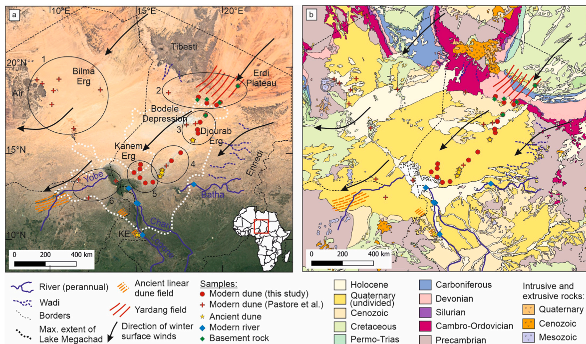
Fig. 1. (a) Main geomorphological features of the southeastern Sahara, with sampling locations for basement rocks, modern river sediment (including one sample from Shellnutt et al., 2019 ), ancient and modern dunes (from this study and from Pastore et al., 2021 ). The location of the figure on the African continent is highlighted by a red square on the African map in the bottom right corner. Winter wind directions from Engelstaedter and Washington (2007) . Max extent of Chad Paleolake from Ghienne et al., (2002) . KE: Kalfou Erg. Circles correspond to sample grouping on Fig. 2 : 1: Bilma Desert; 2: Southern Erdi Plateau; 3: Djourab Desert; 4: Bahr el Ghazal area; 5: Southern Kanem Desert; 6: southern Lake Chad. (b) geological map of the same area ( Persits et al., 1997 ).
