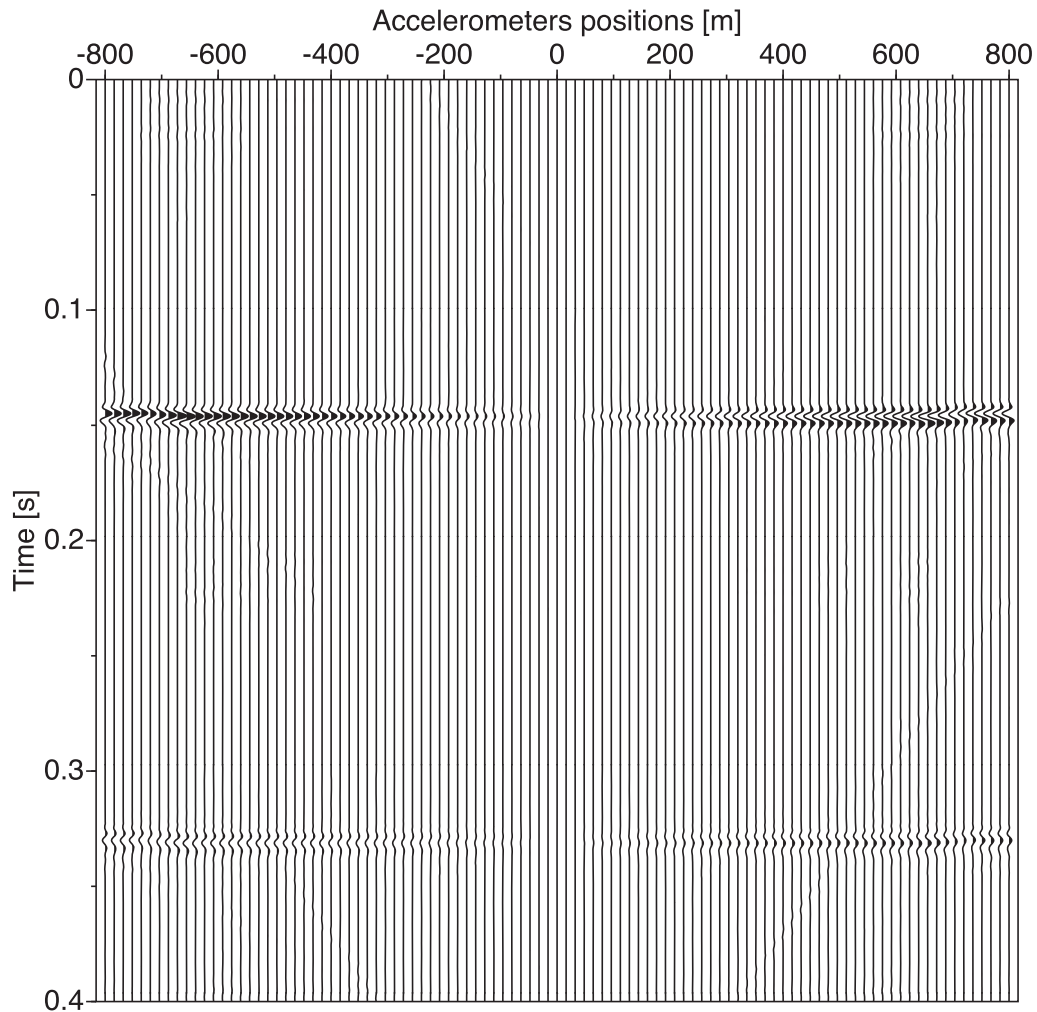
Figure 7. Gather of the vertical component of the seismic wave acceleration \ddot{u}_z , recorded at the surface, considering Model #1. The upwards travelling waves originated at 500 m depth hit the surface at about 0.15 s, at a time compatible with the P -wave velocity, and at about 0.33 s, at a time compatible with the SV-wave velocity.
