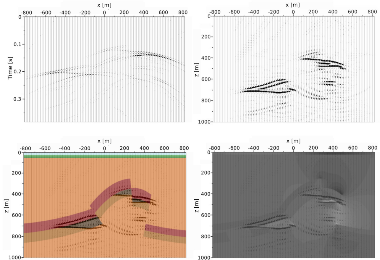
Figure 15. The top left-hand panel depicts the z -component acceleration traces generated by the electroseismic conversion recorded at the surface. The top right-hand panel is the depth migration of these traces. In the bottom panels we show how the migrated seismic data are in agreement with the subsurface model (left-hand panel) and the vertical component of the electric field E_z (right-hand panel).
