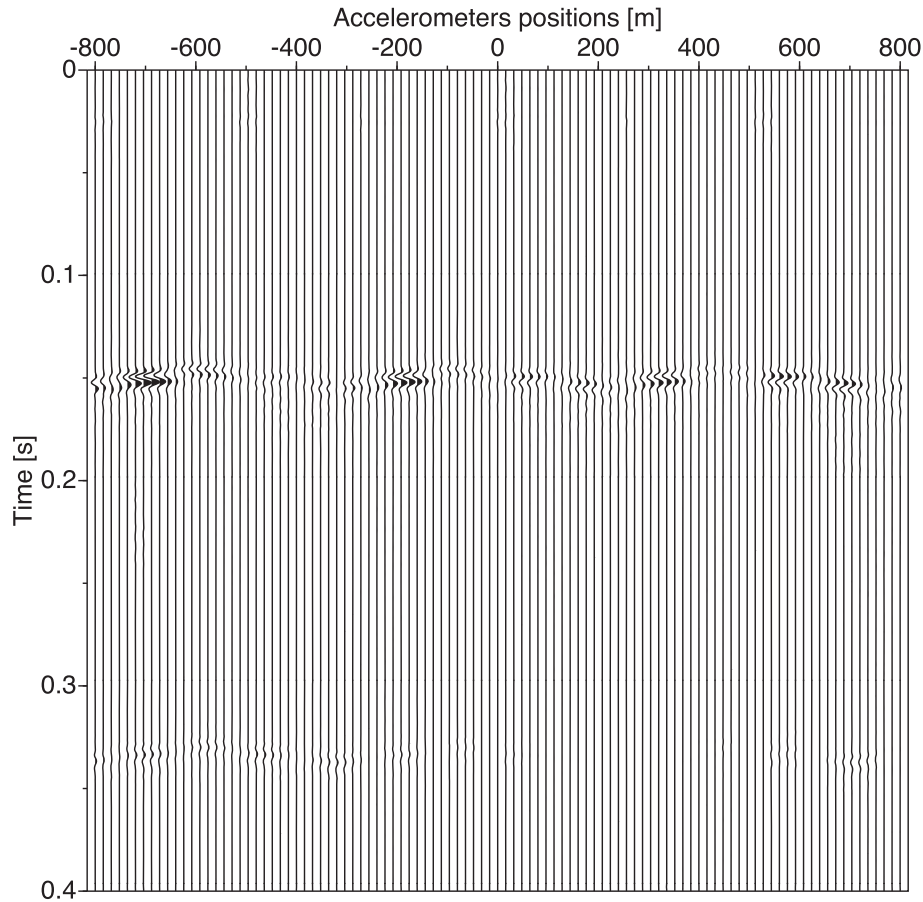
Figure 11. Gather of the vertical component of the seismic wave acceleration \ddot{u}_z , recorded at the surface, considering Model #3. Although the wave fronts originated at the reservoir top are clearly discernible, they are weaker than the ones in Fig. 10, corresponding to Model #2.
