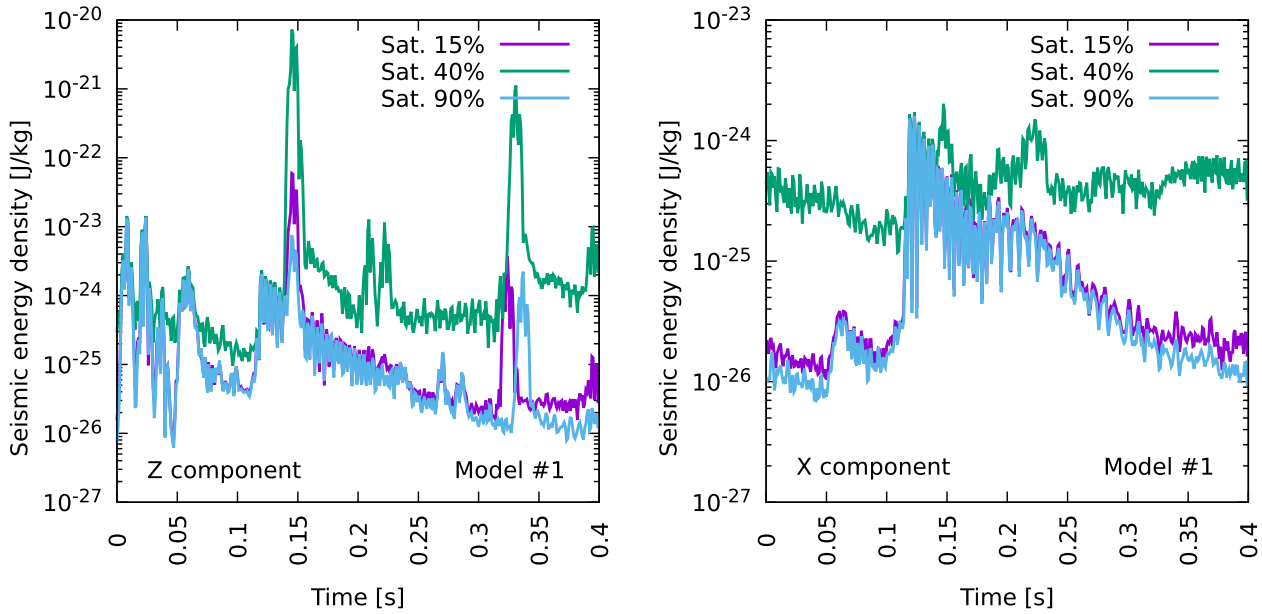
Figure 8. Comparison the seismic energy density for different oil saturations in the reservoir, considering Model #1. The curves are obtained by stacking the squared traces for \dot{u}_z (left-hand panel) and \dot{u}_x (right-hand panel) recorded in all surface receivers, and dividing by the number of receivers.
