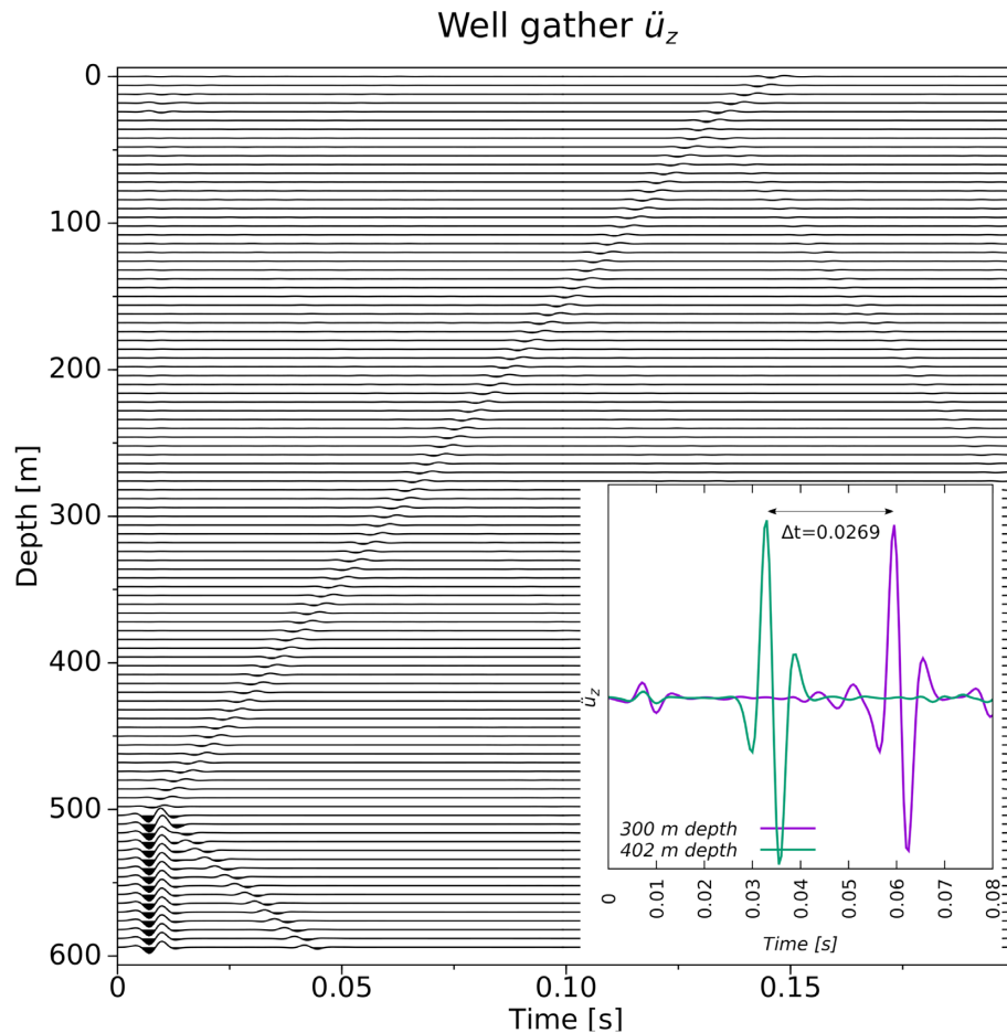
Figure 6. Well gather of the vertical component of the seismic wave acceleration \ddot{u}_z , considering Model #1. The upwards travelling wave originated at 500 m depth hits the surface at about 0.15 s.
