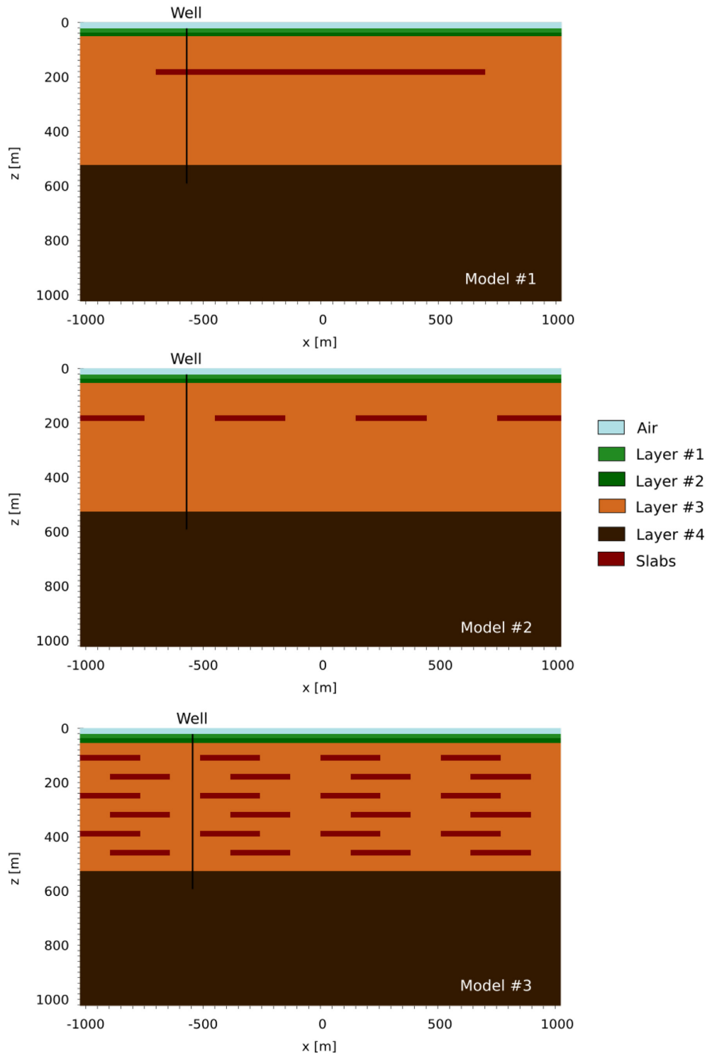
Figure 1. Scaled representation of the first three models analysed in this work. One hundred receivers, from -800 to 800 m separated 16 m from each other are located on the Earth’s surface along the x -direction. In the well, starting at the surface, the same number of receivers is set, separated 6 m from each other. Material properties are described in Table 1.
