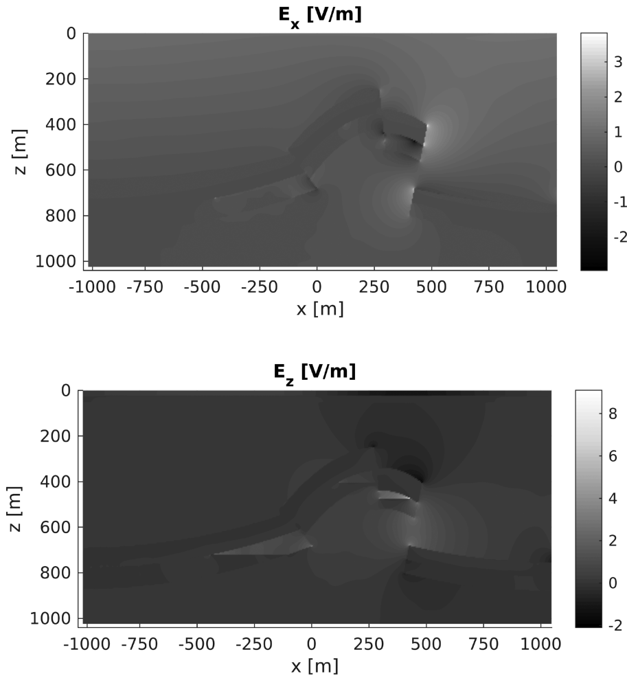
Figure 14. Electric field amplitudes ( E_x top panel, E_z bottom panel), corresponding to a frequency of 120 Hz induced in the discussed model by the plane wave source field, arriving to the earth's surface with the same amplitude ( 1 \text{ V m}^{-1} ) as in the previous models.
