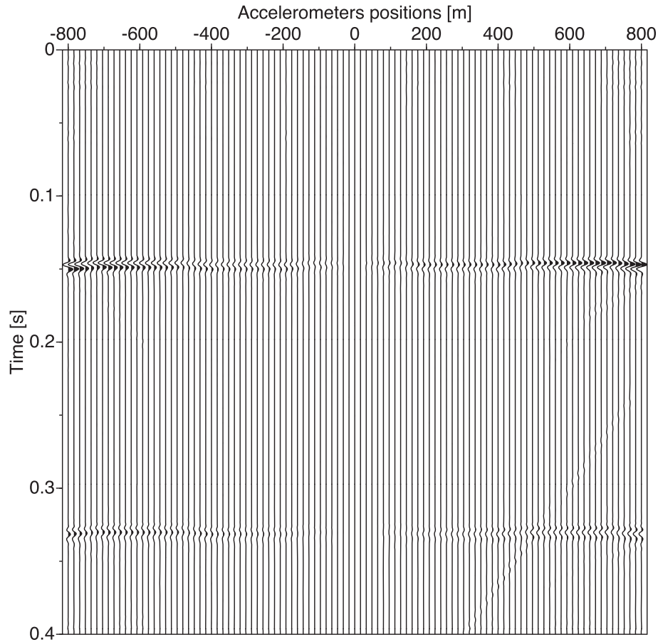
Figure 10. Gather of the vertical component of the seismic wave acceleration \ddot{u}_z , recorded at the surface, considering Model #2. The upwards travelling waves originated at 500 m depth hit the surface at about 0.15 s, at a time compatible with the P wave, and at about 0.33 s, at a time compatible with the SV wave.
