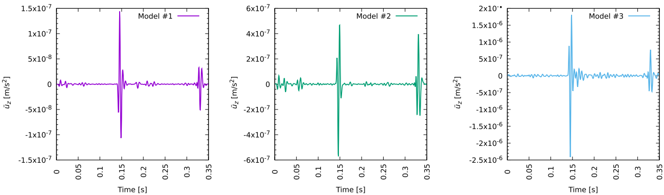
Figure 9. Acceleration traces recorded on the surface ( z component), at the well position, considering Model #1, Model #2 and Model #3. In all cases a 40 per cent oil saturation in the reservoir was considered.
