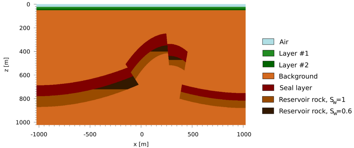
Figure 13. The different structures of this model have the same properties as the ones with the same colours in the previous three models. The water saturated reservoir rock, which is the only new one considered, has the following properties: V_p = 2863 \text{ m s}^{-1} , \sigma = 1.4 \times 10^{-3} \text{ S m}^{-1} , L_0 = 2.1 \times 10^{-10} \text{ A (Pa m)}^{-1} . One hundred receivers, from -800 to 800 \text{ m} separated 16 \text{ m} from each other are located on the Earth's surface along the x -direction.
