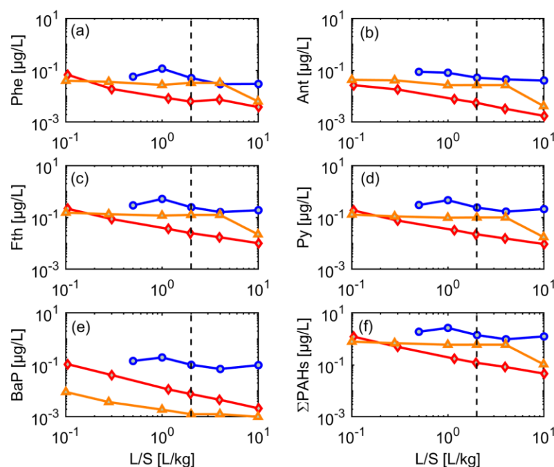
Figure 8. Leaching behavior of selected PAHs from different grain-size fractions of CDW material (CDW3) until a liquid-to-solid (L/S) ratio of 10 (dotted line L/S = 2 ); red diamonds: input material (mixture), blue circles: silt ( <0.063 mm), orange triangles: sand (0–0.2 mm). (a) Phe, (b) Ant, (c) Fth, (d) Py, (e) BaP, and (f) the sum of 16PAHs.
