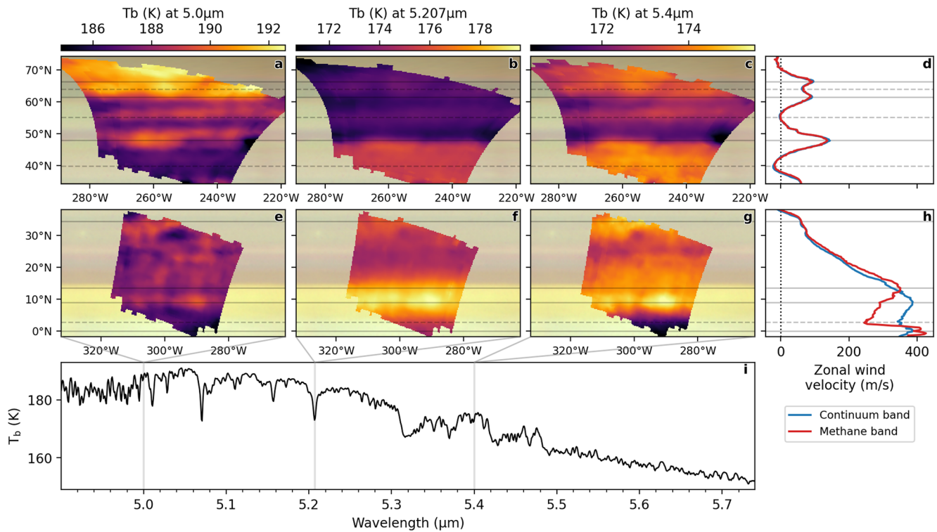
Figure 9. Mapped spatial structure in channel 1-short for low- and mid-latitudes. (d, h) Show the zonal wind velocities (García-Melendo et al., 2011) and (i) shows an example brightness temperature spectrum. While all panels sense a blend of thermal emission and reflected sunlight, panels (a, e) primarily reveal deep thermal emission modulated by overlying aerosol opacity, whereas panels (b, c) and (f, g) primarily reveal reflectivity variations from aerosols in the upper troposphere. Solid and dashed horizontal lines indicate the peaks and troughs of the zonal wind profiles, respectively. The backgrounds of (a–c and e–g) show the color composite map of Saturn created from the HST observations.
