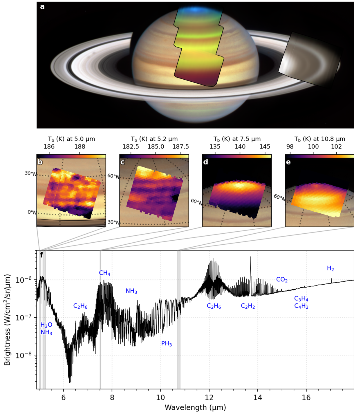
Figure 1. Montage of JWST Mid-Infrared Instrument/Medium Resolution Spectrometer observations of Saturn. Panel (a) shows RGB composites of the JWST observations (Saturn: R = 10.3 \mu\text{m} , G = 10.1 \mu\text{m} , B = 11.6 \mu\text{m} and rings: R = 15.5 \mu\text{m} , G = 14.6 \mu\text{m} , B = 13.5 \mu\text{m} ) with an HST observation of Saturn in the background (Simon et al., 2023). Panels (b–e) show spatial structure on Saturn at a range of wavelengths as indicated by the gray shaded regions in panel (f). (f) Shows the average spectrum of Saturn with specific spectral features labeled.
