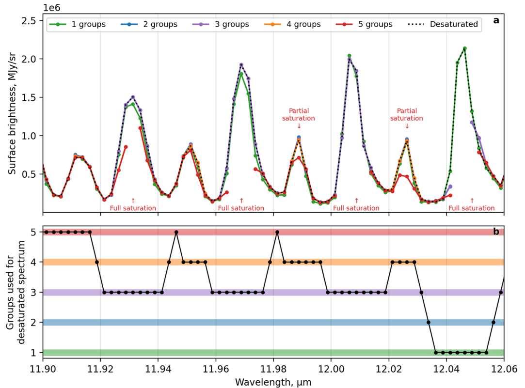
Figure 4. Example spectra showing the desaturation routine. (a) Shows the spectra using different numbers of groups, where the five group data (in red) is the “standard” pipeline output, which shows both saturation and partial saturation. The black dotted line in panel (a) shows the desaturated spectrum which is constructed using a varying number of groups, as shown in panel (b), to minimize saturation while maximizing SNR. The majority of the spectral range uses the full five group data, and only narrow regions (such as this one, in the \nu_9 ethane emission band) require desaturation.
