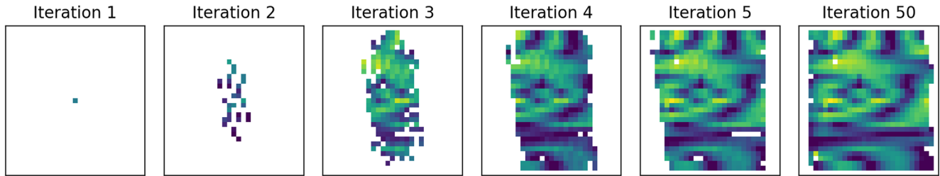
Figure 6. Example flat field at 8.14 \mu\text{m} after the first five iterations of the flat field generation routine, and after the final 50th iteration. The flat is seeded with an initial value for the first iteration, which then uses the corresponding pixel ratios (derived from the dithered observations) to propagate the flat values and fill the image. White pixels have a value of NaN, and the NaN values in the final flat field are regions of the detector that do not contain any data.
