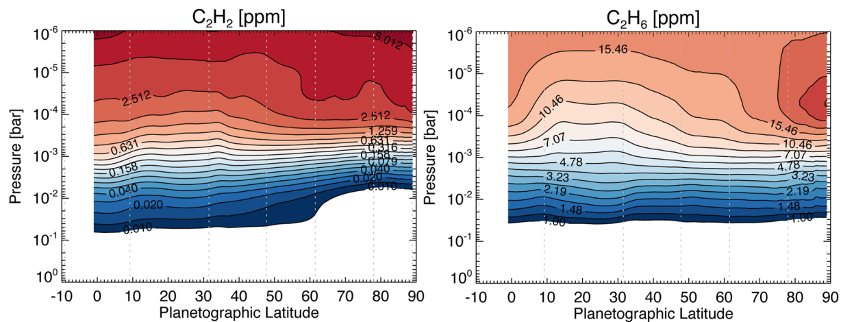
Figure 16. Distributions of acetylene and ethane, derived as continuous profiles to capture changes in the vertical gradients of these species. Contours are logarithmic, and labeled in ppmv. Vertical dotted lines show the latitudes of tropospheric eastward jets. A cross-section at 0.5 mbar is shown in Figure 17.
