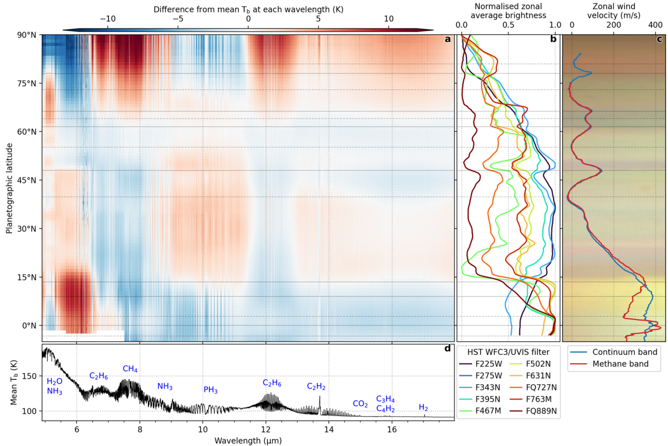
Figure 8. Variation in Saturn's zonal average brightness temperature with wavelength and latitude. (a) Shows the difference from the mean brightness temperature spectrum (d), where red areas are brighter than the average and blue areas are dimmer. (b) Shows the normalized zonal average brightness of HST observations of Saturn in September 2022 (Simon et al., 2023) and (c) shows Saturn's zonal wind profiles (García-Melendo et al., 2011). Solid and dashed horizontal lines in panels (a–c) indicate the peaks and troughs of the zonal wind profiles, respectively. The background of panel (c) shows part of the color composite map of Saturn created from the HST observations.
