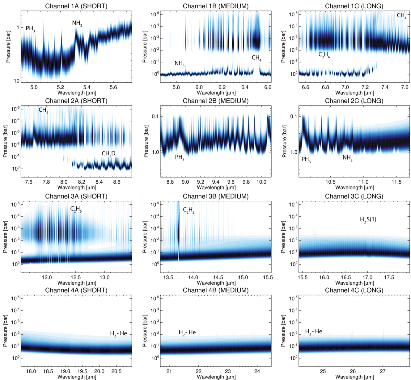
Figure 13. Cloud-free contribution functions (Jacobians showing the rate of change of spectral radiance with temperature) calculated for nadir viewing and a typical mid-latitude composition on Saturn. These contribution functions have been normalized at each wavelength, and darker shading indicates the greatest contribution. No aerosols are included in this model. Key gaseous features have been labeled, note that minor stratospheric species become apparent with higher emission angles (not shown). The y-axis changes in pressure range to emphasize dominant features.
