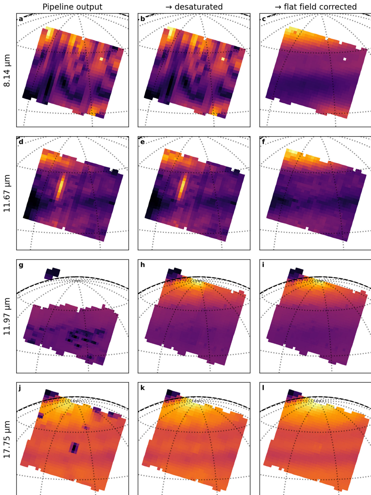
Figure 3. Example cube slices at different stages of our custom Mid-Infrared Instrument data reduction process. The first column shows the output of the standard JWST pipeline, which still contains significant flat field effects (a and d), saturation (g), and partial saturation (dark pixels in panels (g and j)). The second column shows the data after the desaturation step is applied and the third column shows the data after the flat field correction is applied.
