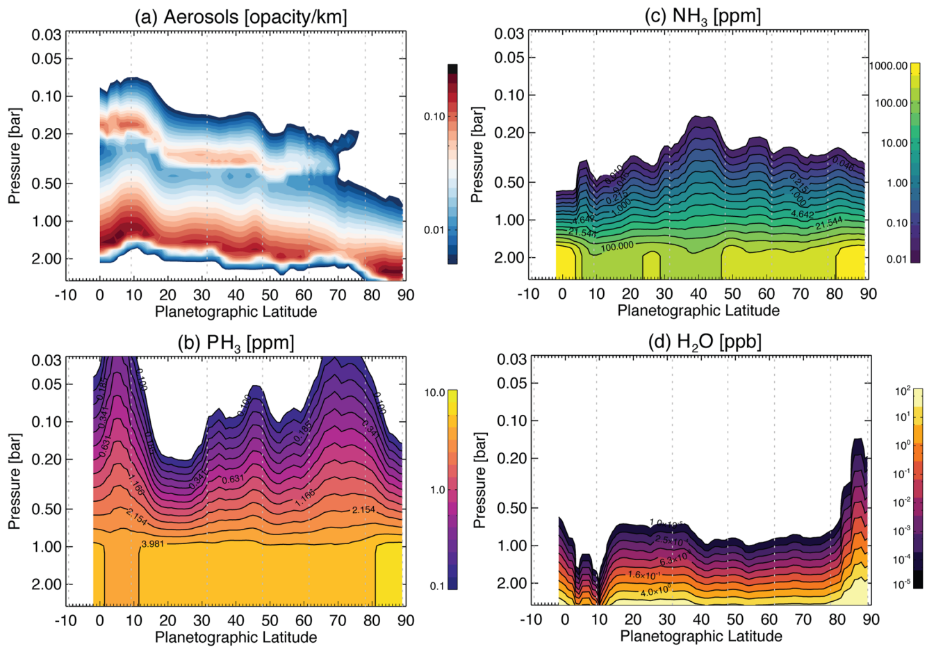
Figure 15. Aerosols, phosphine, ammonia, and water derived from the 4.9–7.3 \mu\text{m} region. Aerosols in panel (a) are plotted in opacity/km at a reference wavelength of 5 \mu\text{m} , calculated following the scheme in Appendix C of Irwin et al. (2022). A logarithmic color bar is used to show structure within the aerosol cross-section. For the gases in panels (b–d), the contours are also logarithmic to allow for the rapid decline of the abundance with altitude. \text{PH}_3 and \text{NH}_3 are provided in ppm, \text{H}_2\text{O} is given in ppb. Vertical dotted lines show the latitudes of tropospheric eastward jets.
