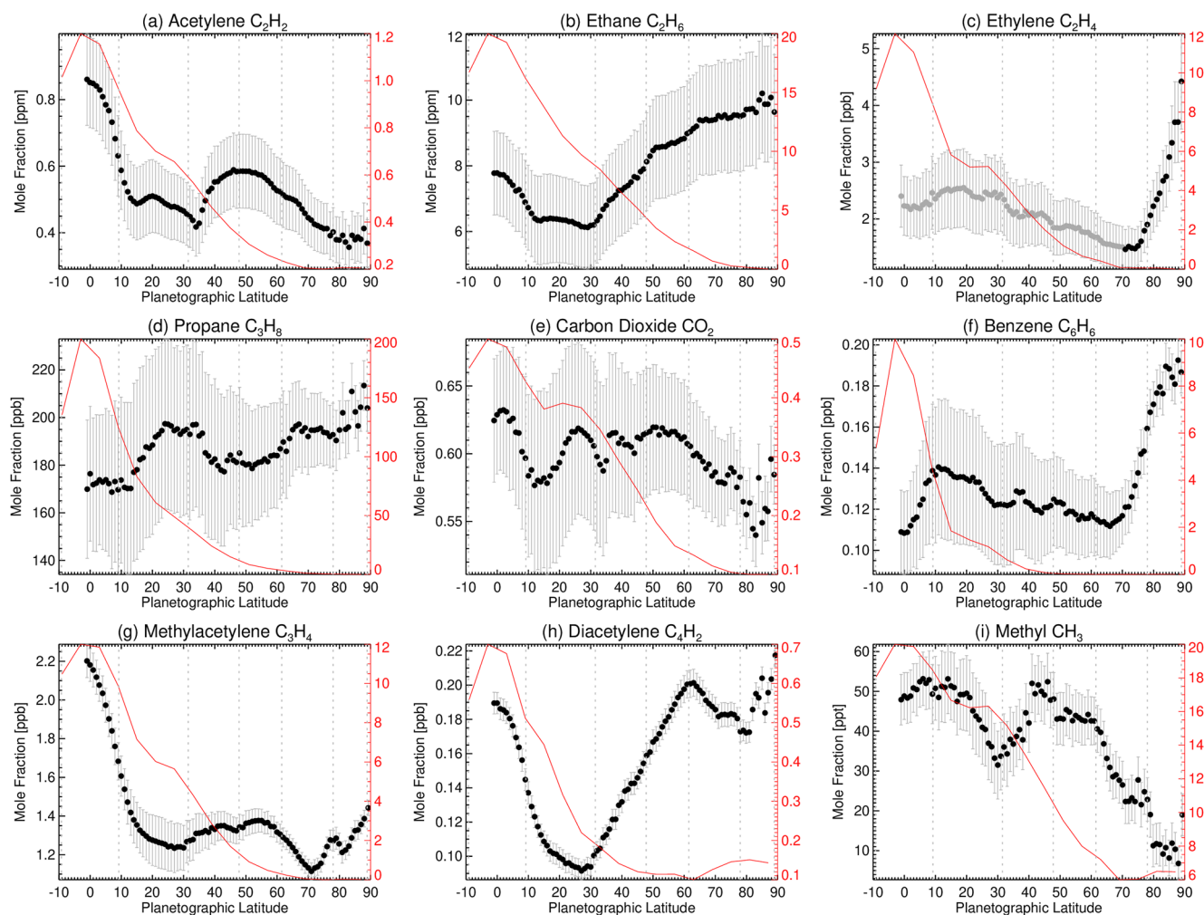
Figure 17. Distributions of stratospheric species at 0.5 mbar: acetylene, ethane, ethylene, propane, \text{CO}_2 , benzene, methylacetylene (propyne), diacetylene (1,3-butadiyne), and methyl in Saturn's northern summer, compared to the predictions of the neutral photochemistry model for L_s = 150^\circ (Moses & Greathouse, 2005; Moses et al., 2007). The photochemical model is shown in red, and is referenced to the right-hand axis so that both the shape of the distribution and differences in absolute abundances can be compared. Error bars are shown in gray, but these do not include uncertainties due to scaling a latitudinally uniform a priori profile. If the shape of the profile changes significantly with latitude (as is expected for benzene and \text{C}_4\text{H}_2 from previous studies), this could influence the retrieved values. Vertical dotted lines show the latitudes of tropospheric eastward jets. Gases in panels (a–c) were derived as full vertical profiles, other gases are derived as scale factors for our a priori profiles. Gray points in panel (c) signify a lack of obvious detection of \text{C}_2\text{H}_4 emission by eye.
