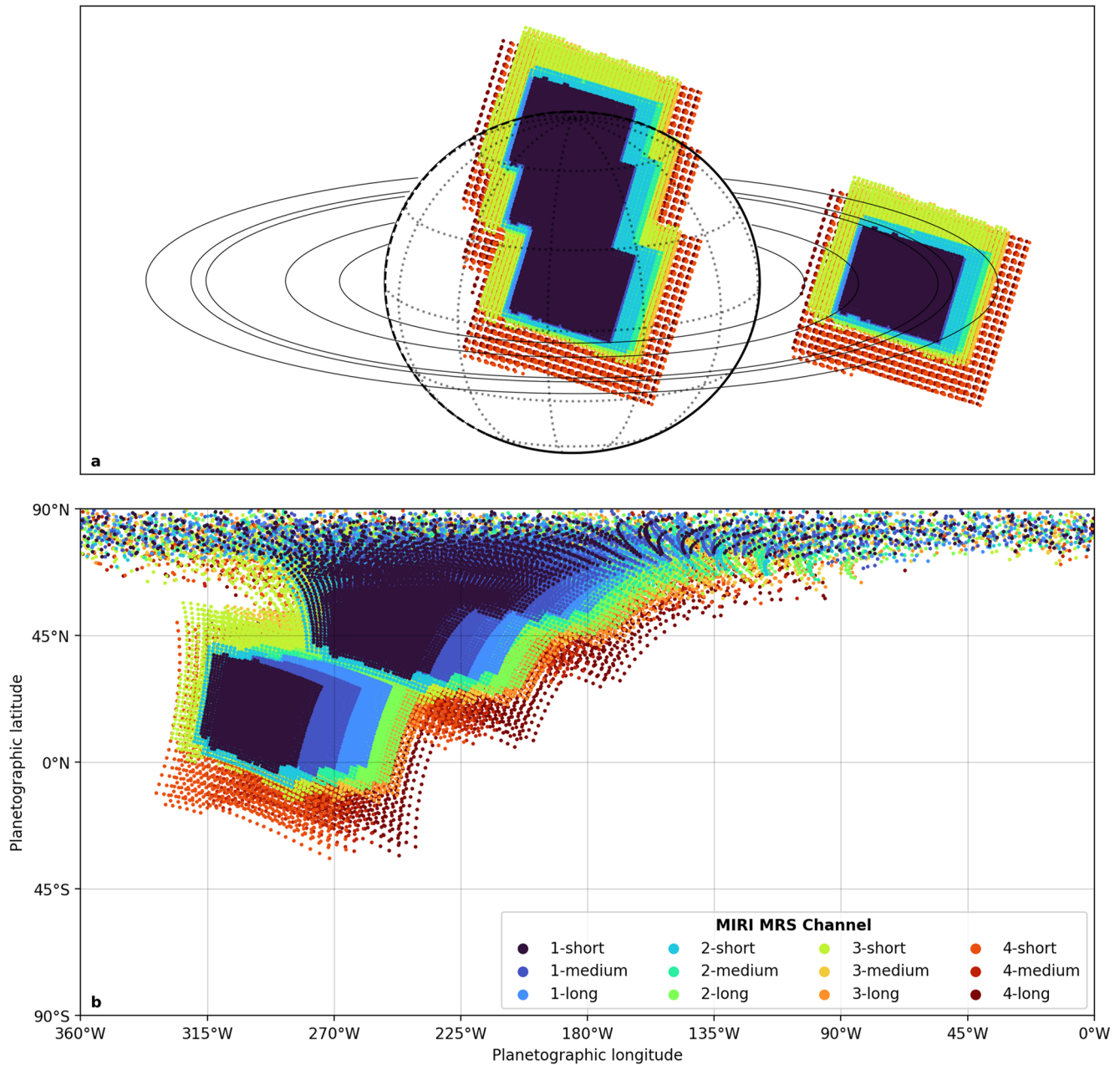
Figure 2. Spatial coverage of Mid-Infrared Instrument (MIRI) observations (a) relative to Saturn's disc and (b) mapped to Saturn's surface. Each dot represents the location of a single spaxel with the color indicating the MIRI channel. The background observation was located 90" to the north of Saturn, so is not shown here (Saturn's disc has a diameter of ~17").
