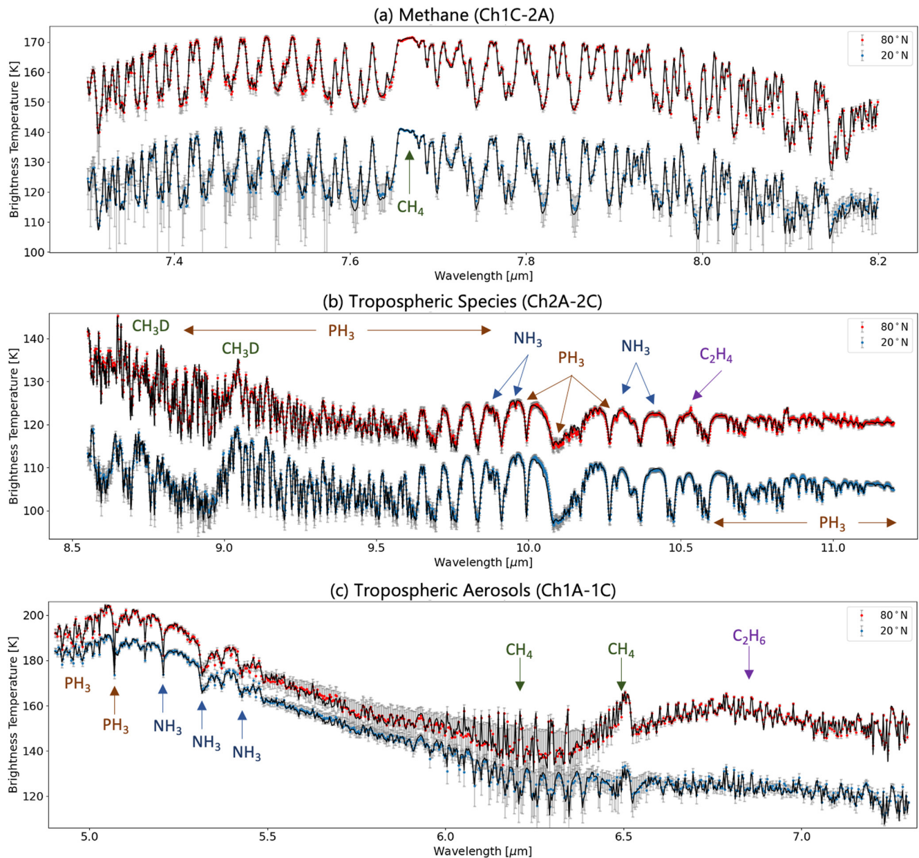
Figure 11. Examples of the quality of spectral fits (solid lines) to Mid-Infrared Instrument/Medium Resolution Spectrometer data (points with error bars) at different stages within our multi-stage retrieval. Panel (a) is dominated by stratospheric \text{CH}_4 emission, used to determine the vertical temperature structure; panel (b) sounds tropospheric species like \text{PH}_3 , \text{NH}_3 , and \text{CH}_3\text{D} ; panel (c) sounds reflection and absorption by tropospheric aerosols, in addition to \text{PH}_3 , \text{NH}_3 , \text{H}_2\text{O} , and emission from stratospheric \text{CH}_4 and \text{C}_2\text{H}_2 . Spectra at 80°N have been offset from the 20°N spectra by 20 K for clarity. Uncertainties are a scaled version of those reported by the JWST pipeline, as described in Section 4.
