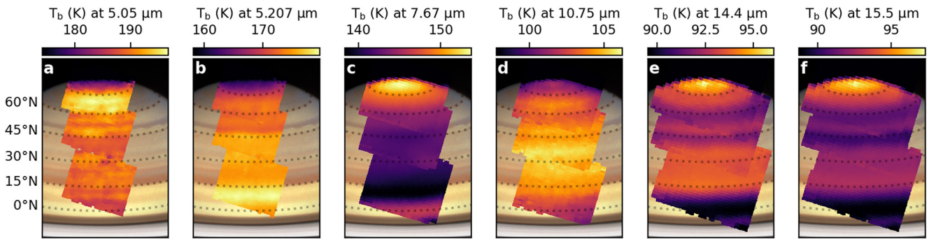
Figure 7. Composite images created by combining all three Saturn tiles to show the equator-to-pole variation in brightness temperature at different wavelengths. 5.05 \mu\text{m} senses aerosol opacity in the deep troposphere (3–6 bars), whereas 5.207 \mu\text{m} is in a strong \text{NH}_3 absorption and senses a blend of thermal emission and reflected sunlight from upper tropospheric aerosols. 7.67 \mu\text{m} senses stratospheric temperatures (0.1–5 mbar) via \text{CH}_4 emission; whereas 10.75 \mu\text{m} senses a blend of tropospheric temperature and ammonia opacity near 400–600 mbars. 14.4 and 15.5 \mu\text{m} are primarily sensitive to the \text{H}_2 -He continuum, sounding tropospheric temperatures in the 100–300-mbar range. Note that each tile observed a different longitude range, but are shown overlapping here for simplicity—this causes some artificial inconsistencies in brightness at regions of overlap.
