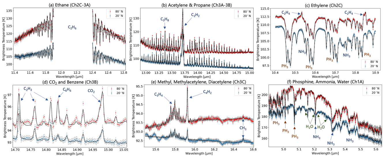
Figure 12. Example fits (black line) to observations (points with error bars) in specific regions of Saturn's spectrum, including those regions sensing stratospheric hydrocarbons (ethane in panel (a) with the central region omitted as described in the text; acetylene and propane in panel (b); ethylene in panel (c); CO 2 and benzene in panel (d); and methylacetylene, diacetylene, and methyl in panel (e)) and tropospheric absorptions from ammonia, phosphine, and (tentatively) water in panels (c, f). Spectra for 80°N have been offset from 20°N for clarity by 10 K in panels (a, c); 20 K in panels (b, f)—no offsets were used in panels (d, e).
