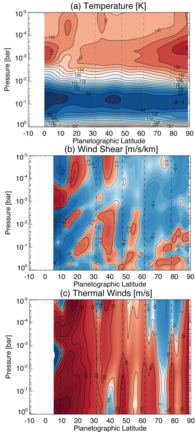
Figure 14. Temperatures, windshear, and thermal winds as a function of latitude derived from Mid-Infrared Instrument/ Medium Resolution Spectrometer spectroscopy. The peaks of cloud-tracked eastward winds are shown as vertical dashed lines for context. In panels (b, c), regions of negative windshear/westward winds are shown as blue with dotted contours; regions of positive windshear/eastward winds are shown as red with solid contours. Temperature contours are every 4 K; windshear and wind contours are logarithmic to show structure, but windshears are labeled at \pm 0.1 , \pm 0.5 , and \pm 1.0 m/s/km; winds are labeled at 10, 50, 100, 150, and 200 m/s. Absolute values for derived thermal winds are subject to significant uncertainties related to the integration of the thermal wind equation (Fletcher et al., 2016), so should be used as a guideline to trends only.
