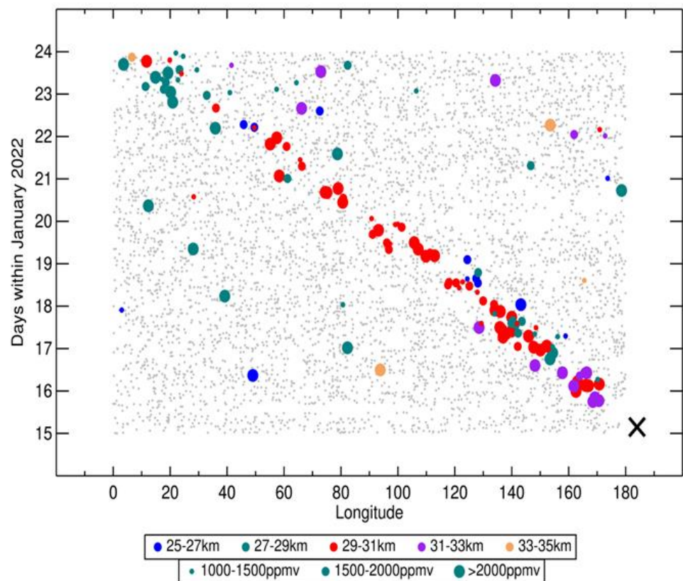
Figure 6. Longitude vs. time diagram showing locations of H 2 O profiles with maximum values >1000 ppmv over 25–35 km, over the domain 10–30°S, for the first week following the HTHH eruption (noted by the 'X' on 15 January). The colors and symbols denote the altitudes and concentrations of the H 2 O maxima. The grey dots indicate all of the C2 measurement locations.
