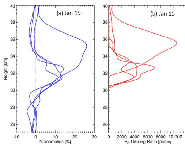
Figure 4. Vertical profiles of (a) refractivity anomaly and (b) derived H 2 O mixing ratios for C2 observations within the HTHH plume on 15 January. Most of these N profiles are associated with a ‘bad’ flag in the retrieval, although the structures are reasonable and may be consistent with actual geophysical information.
