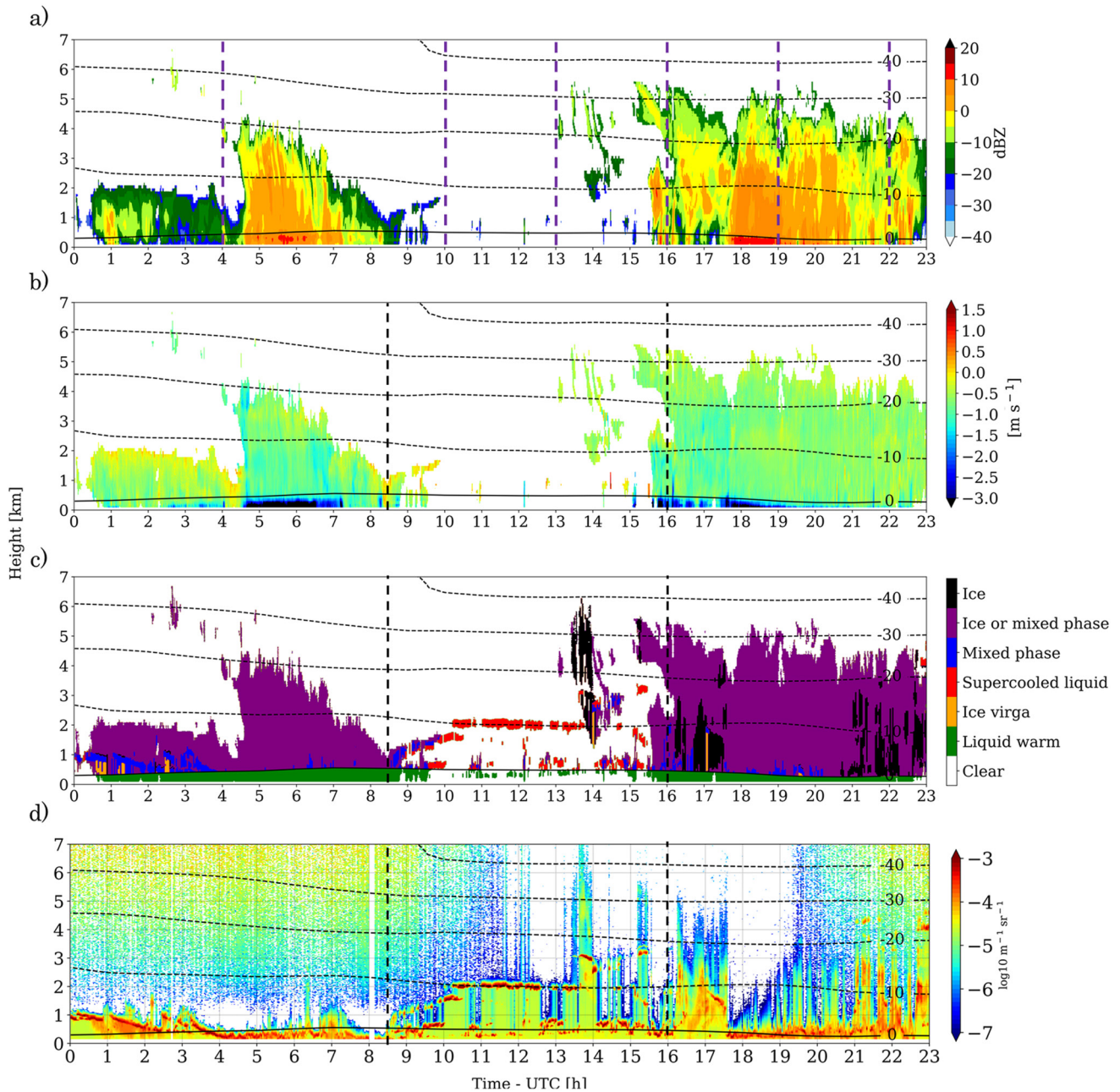
Figure 4. Time height plots of (a) the 95 GHz radar reflectivity dBZ from BASTA, (b) Doppler velocity ( V_{\text{Doppler}} ), (c) Cloud phase from the merged cloud radar and lidar and (d) cross-section of lidar attenuated backscatter aboard the RV Investigator on 16 Feb 2018. Dashed black contours indicate the air temperature from ERA5 (10°C intervals). Vertical dashed purple in (a) and black lines in (b)–(d) indicate the sounding launch times and the approximate time of the three meteorological events, respectively.
