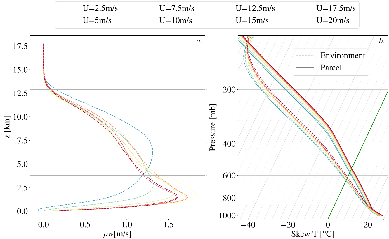
Figure 5. (a) Mass flux profiles ( \rho w ) for all cases, computed for high condensate columns (beyond 99.9th). The control case ( U_{sf} = 2.5 m/s), in blue, is a near parabolic profile, and as the shear increases we observe profiles becoming more “bottom heavy,” consistent with Abbott et al. (2020). The mass flux at the boundary layer increase until the optimal regime and slowly decrease in the superoptimal regime. (b) Environment temperature profile, averaged near an extreme of CAPE (beyond 99.9th) in dashed lines, and adiabatic parcel ascent in solid lines are displayed in Skew-T diagrams. The CAPE for each case is read as the area between two profiles of same color. This graph highlights the low sensitivity of the CAPE to shear changes across simulation experiments.
