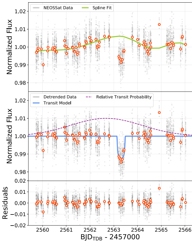
Figure 4. A week-long observation by NEOSat. Gaps in the light curve are due to Earth eclipse and other necessary telescope operations. The star was imaged with a cadence of 23 s while on target. Displayed bins are 60 minutes. Top: a KEPLERSPLINE fit to the out-of-transit region to model systematics (discussed in Section 3.3). Middle: the transit fitted to the corrected light curve. The dashed purple curve shows relative probability of the expected transit based on the RV-derived period constraints available at the time of observation. Bottom: residuals of the transit fit.
