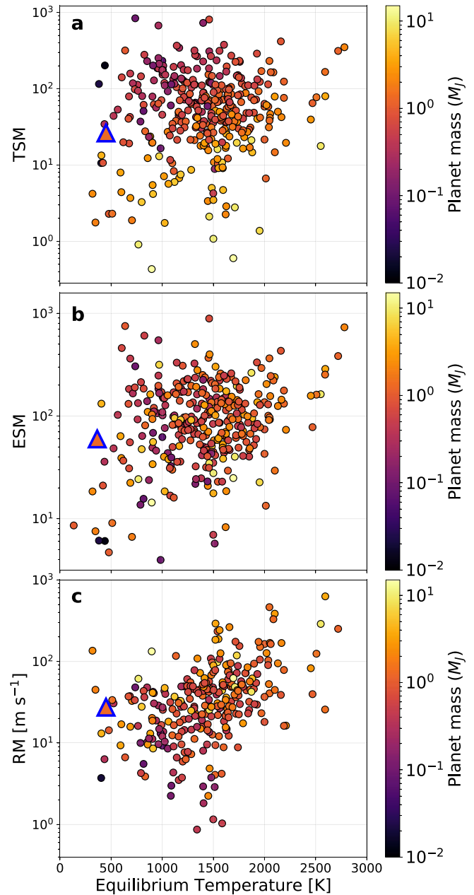
Figure 10. Comparison of expected signal strengths for the same planet population shown in Figure 9. TOI-2010 b is indicated with the triangle marker. Panel (a): TSM. The TSM provides an S/N estimate for a JWST/NIRISS transit observation. Panel (b): ESM. The ESM provides an S/N estimate for a JWST/MIRI eclipse observation. Panel (c): RM signal amplitude. The TOI-2010 b value in this plot uses v \sin i_* = 2.8 \text{ km s}^{-1} , derived from the TESS and WASP light-curve modulations.
