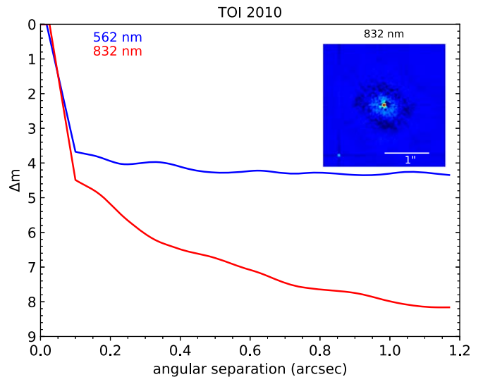
Figure 2. Contrast curves from Gemini-N/‘Alopeke speckle image. Curves show the 5\sigma contrast limit. The faint source in the lower left of the inset image is a previously unresolved neighbor star not present in the Gaia DR3 catalog.
