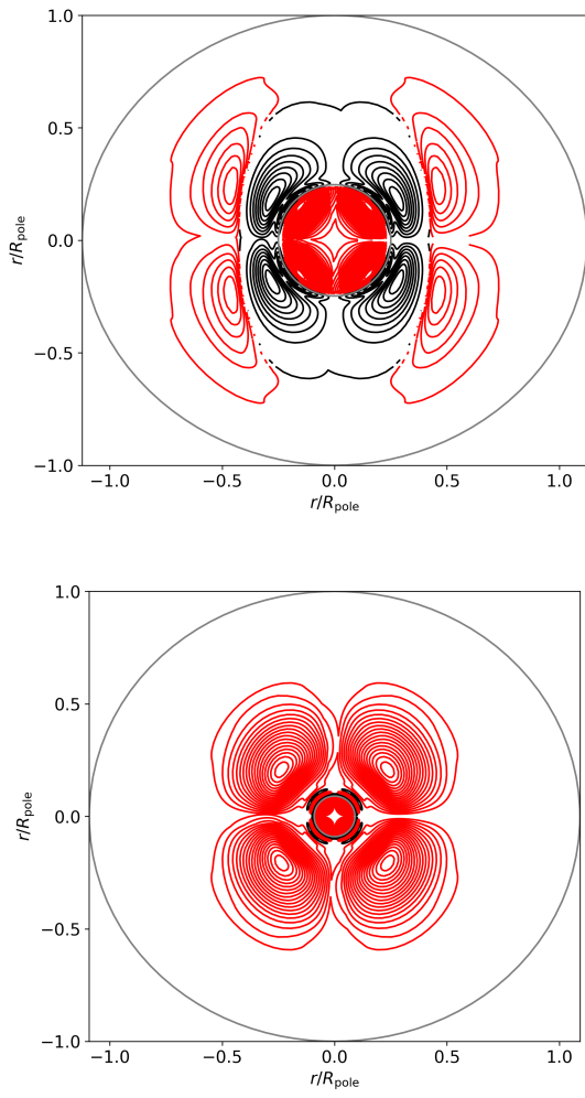
Fig. E.2. Same as Fig E.1, but for model M2.
