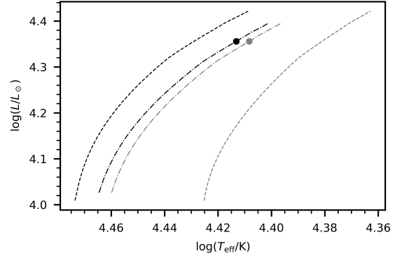
Fig. 1. HRD showing the evolution tracks of the 2D models for a 12 M_{\odot} star ( Z = 0.012 , X_i = 0.71 ) for (\Omega_{\text{eq}}/\Omega_{\text{c}})_i = 0.15 (dashed-dotted), and 0.5 (dashed). The black lines represent the properties at the pole, the grey lines the properties at the equator. The tracks are terminated slightly before the TAMS when the solver can no longer converge, which occurs at X_c/X_{\text{ini}} = 0.141 and 0.131 for the respective aforementioned rotation rates. The dots mark the model of HD 192575 that is discussed in Sect. 3.
