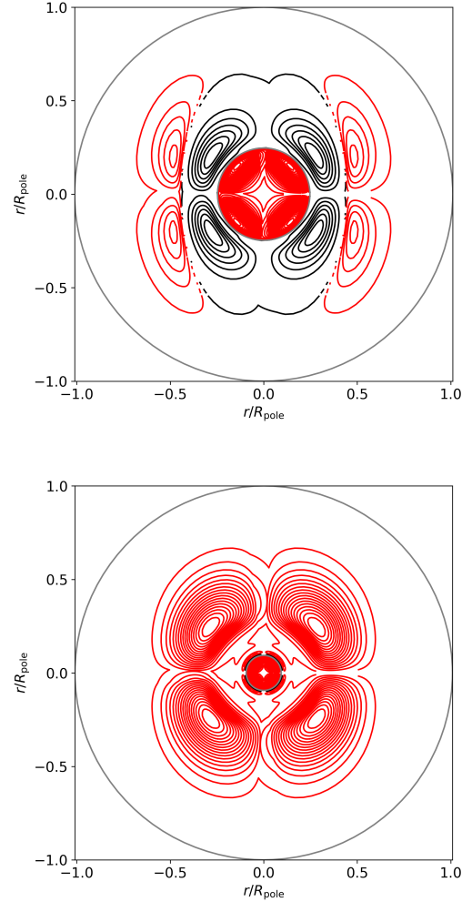
Fig. E.1. Isocontours of the stream function for model M1 of 1 Myr (top panel) and 15.75 Myr (bottom panel). The different colours indicate counter-rotating cells, where the red cells rotate clockwise in the first quadrant of the plot. These models correspond to those shown in Fig. 2. The isobars at the edge of the convective core and at the surface are shown in grey.
