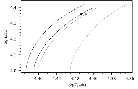
Fig. 1. HRD showing the evolution tracks of the 2D models for a 12 M_{\odot} star ( Z = 0.012 , X_i = 0.71 ) for (\Omega_{\text{eq}}/\Omega_c)_i = 0.15 (dashed-dotted), and 0.5 (dashed). The black lines represent the properties at the pole, the grey lines the properties at the equator. The tracks are terminated slightly before the TAMS when the solver can no longer converge, which occurs at X_c/X_{\text{ini}} = 0.141 and 0.131 for the respective aforementioned rotation rates. The dots mark the model of HD 192575 that is discussed in Sect. 3.
