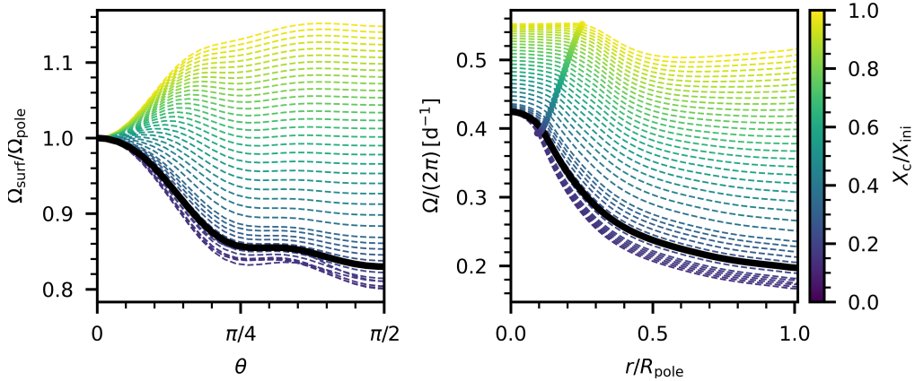
Fig. 4. Evolution of the rotation profile of model M1. Left panel: predicted surface rotation as a function of colatitude throughout the evolution (indicated by colour) normalised by the rotation frequency at the pole. Right panel: profile of the angular velocity (averaged over \theta ) throughout the evolution. The thick coloured line indicates the location of the convective core boundary. The black lines in both panels correspond to the best-matching model for HD 192575 (last column in Table 1).
