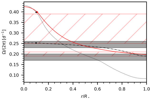
Fig. 5. Predicted rotation profile of HD 192575 with ESTER (red solid line) and MESA (black lines). The profiles indicated by a solid line and dotted line are for a constant viscosity of 10^7 \text{ cm}^2 \text{ s}^{-1} , while the dashed line is for 10^9 \text{ cm}^2 \text{ s}^{-1} . The dots correspond to the location of the core boundary. The red and grey shaded areas indicate the measured core (top one) and surface (bottom one) rotation frequencies by Burssens et al. (2023), assuming r_{\text{shear}} equal to the outer boundary of the \mu -gradient zone, and r_{\text{shear}} = R_* , respectively.
