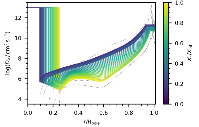
Fig. 3. Profile of the vertical diffusion coefficient according to Eq. (2) for a 12 M_{\odot} model with an initial rotation frequency of 15% the critical angular velocity. The grey dotted lines show D_v(N_0^2)_v/(\eta N^2) at a few ages (from left to right: X_c/X_{\text{ini}} = 0.14, 0.30, 0.58, 0.82, 0.98 ), that is, if we were to take the local value of the Brunt-Väisälä frequency instead of the volume averaged value.
