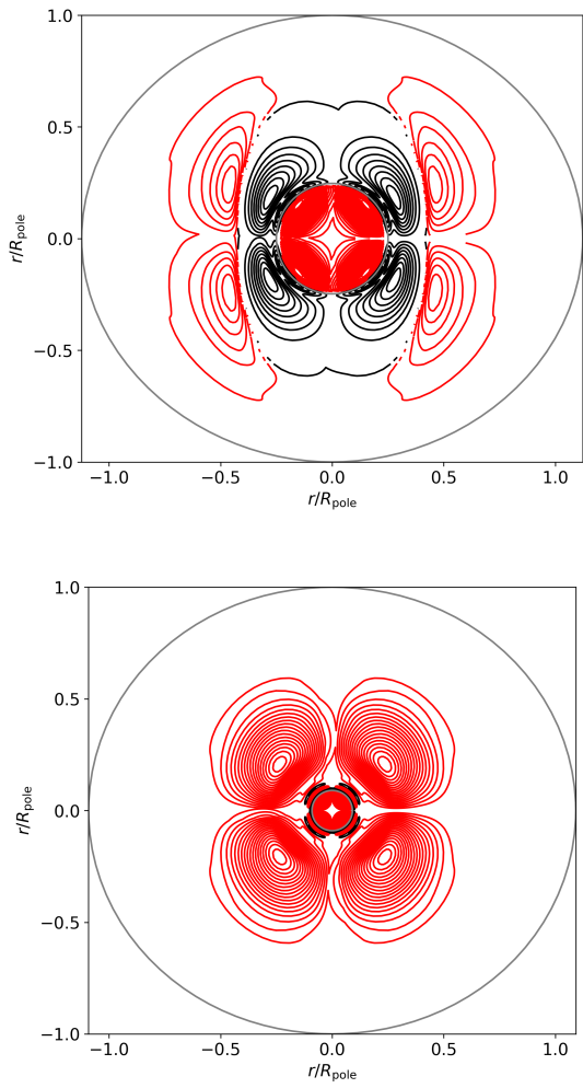
Fig. E.2. Same as Fig E.1, but for model M2.
