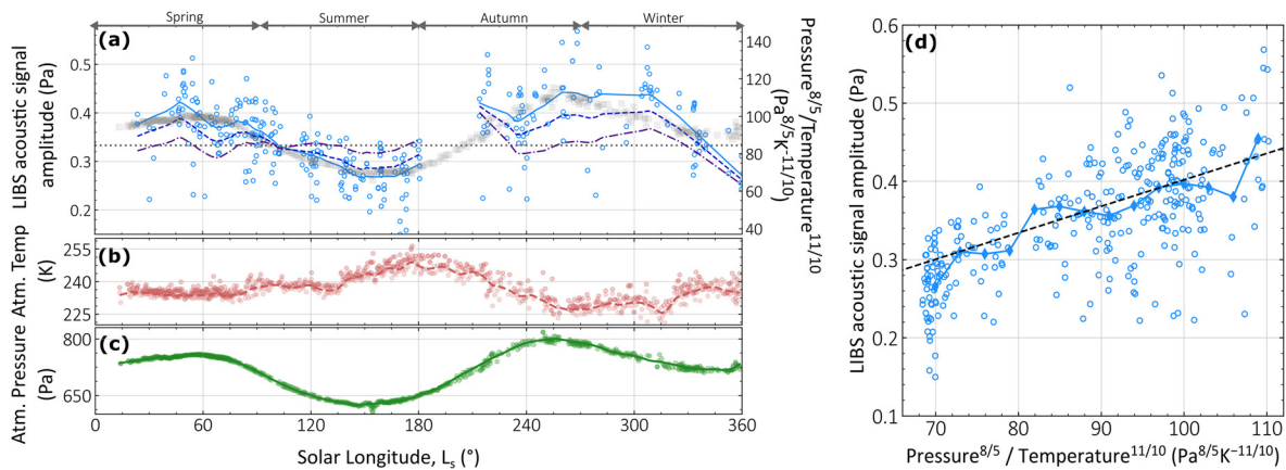
Fig. 3. (a) Seasonal evolution of the LIBS acoustic signal amplitude between 11:00 and 14:00 LTST (blue points). The solid light blue line represents a smoothing over 30^\circ of solar longitude. This smoothed trend is subsequently corrected for the Rankine-Hugoniot shock condition (dark blue, dashed) and for the acoustic impedance variation (purple, dashed-dotted) – see text. Both corrections are normalized to a temperature of 240 K and a pressure of 700 Pa (i.e., atmospheric conditions at L_s = 90^\circ ). The data are superimposed with the seasonal variation of the ratio P^{8/5}/T^{11/10} (gray squares), which comes from the theory described in Equation (13) and is computed from the data in panels b and c. The dotted horizontal line corresponds to the median corrected amplitude. (b) Seasonal evolution of air temperature at a height of 1.5 m at 12:00 LTST. (c) Seasonal evolution of atmospheric pressure at 12:00 LTST. (d) Correlation between the LIBS acoustic signal amplitude normalized to a distance of 2 m and P^{8/5}/T^{11/10} computed with the MEDA data for each acoustic point. Circles represent all the data points whereas diamonds represent a running mean subset.
