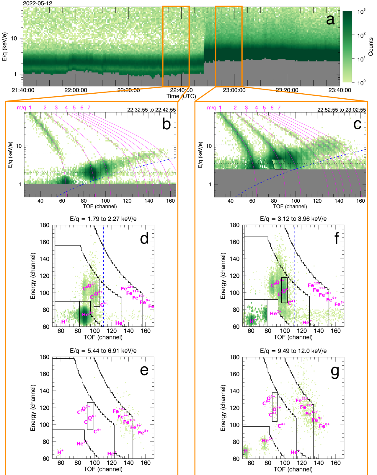
Fig. 2. HIS measurements about an interplanetary shock encountered by Solar Orbiter on 12 May 2022. Panel (a): HIS E/q spectra at native 30-s resolution over a 2 h interval. Panels (b),(c): E/q-TOF distributions accumulated over 10-min before and after the shock, corresponding respectively to the orange-outlined intervals in panel (a). Panels (d)–(g): E-TOF distributions at the peak E/q step for He 2+ and other M/q = 2 ions (panels (d),(f)) and for Fe 9+ (panels (e),(g)). The colorbar is consistent throughout all panels. Dark gray indicates E/q steps affected by the instrument’s proton avoidance (panels (a),(c)), magenta corresponds to m/q (panels (b),(c)) and ion species (panels (d)–(g)), dashed blue lines are the velocity filter applied to the data panels (b)–(g), and thick black lines mark boundaries between priority ranges as listed in Table 1 panels (c)–(g). Suprathermal trails for (left to right in TOF) H + , He 2+ , and He 1+ can be observed in panels (b),(c).
