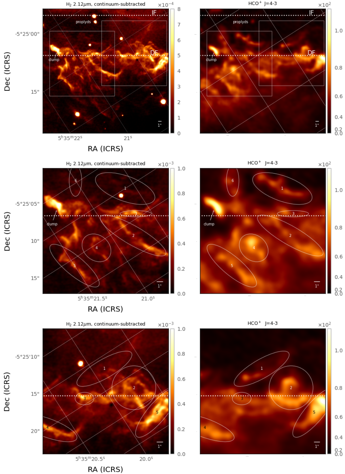
Fig. 6. Left panels: integrated intensity maps (continuum-subtracted) of the H 2 1–0 S(1) line emission in \text{erg cm}^{-2} \text{s}^{-1} \text{sr}^{-1} . Right panels: integrated intensity maps of the HCO + J = 4-3 lines in \text{K km s}^{-1} .
