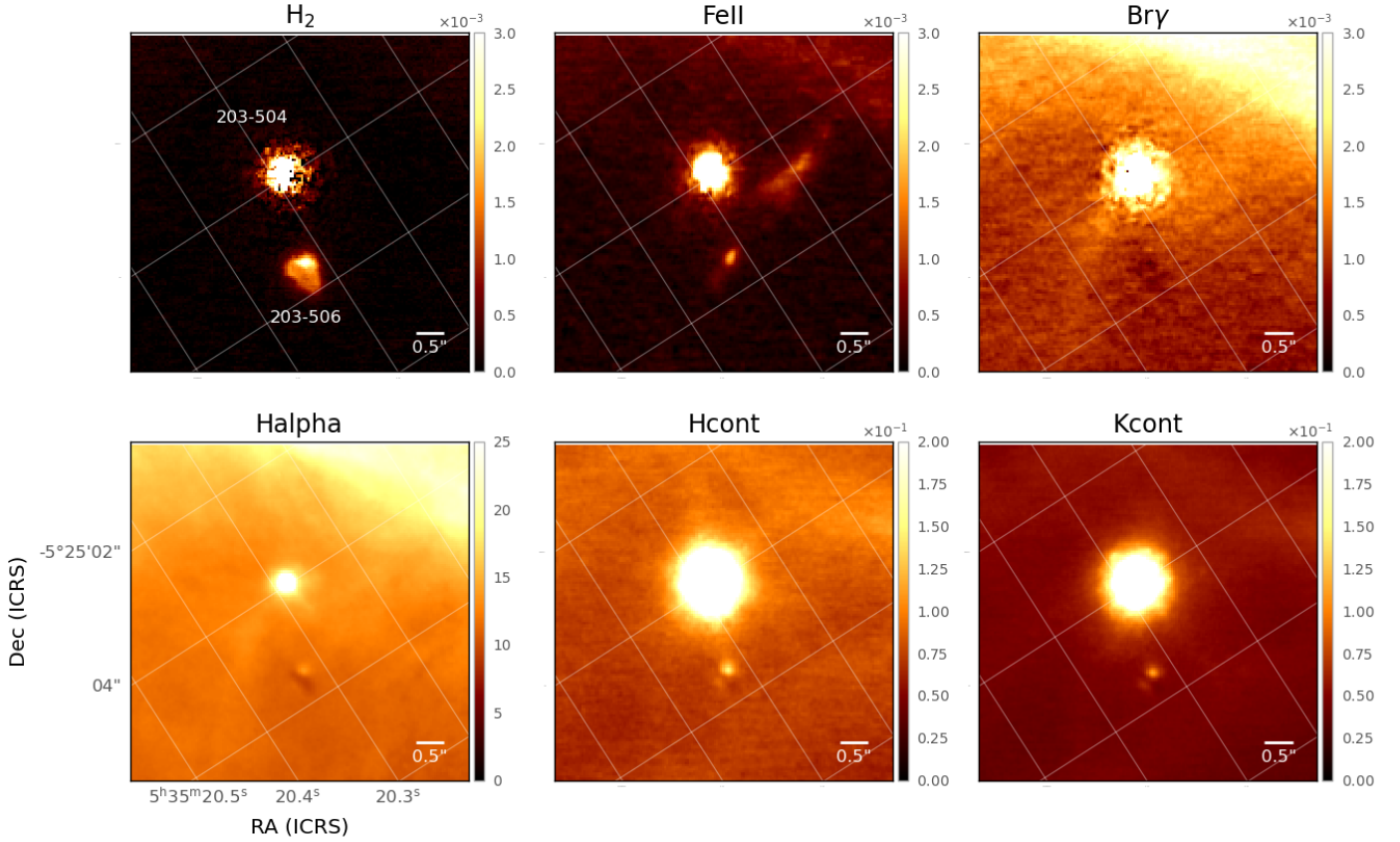
Fig. 7. Zoom into proplyds in the H 2 2.12 \mu\text{m} , [FeII] 1.64 \mu\text{m} , and Br \gamma 2.16 \mu\text{m} lines (continuum subtracted), as well as, in the Hcont and Kcont filters with the H \alpha emission in addition using the HST observations from https://archive.stsci.edu/prepds/orion/acs_displaypage.html which was adjusted in positions.
