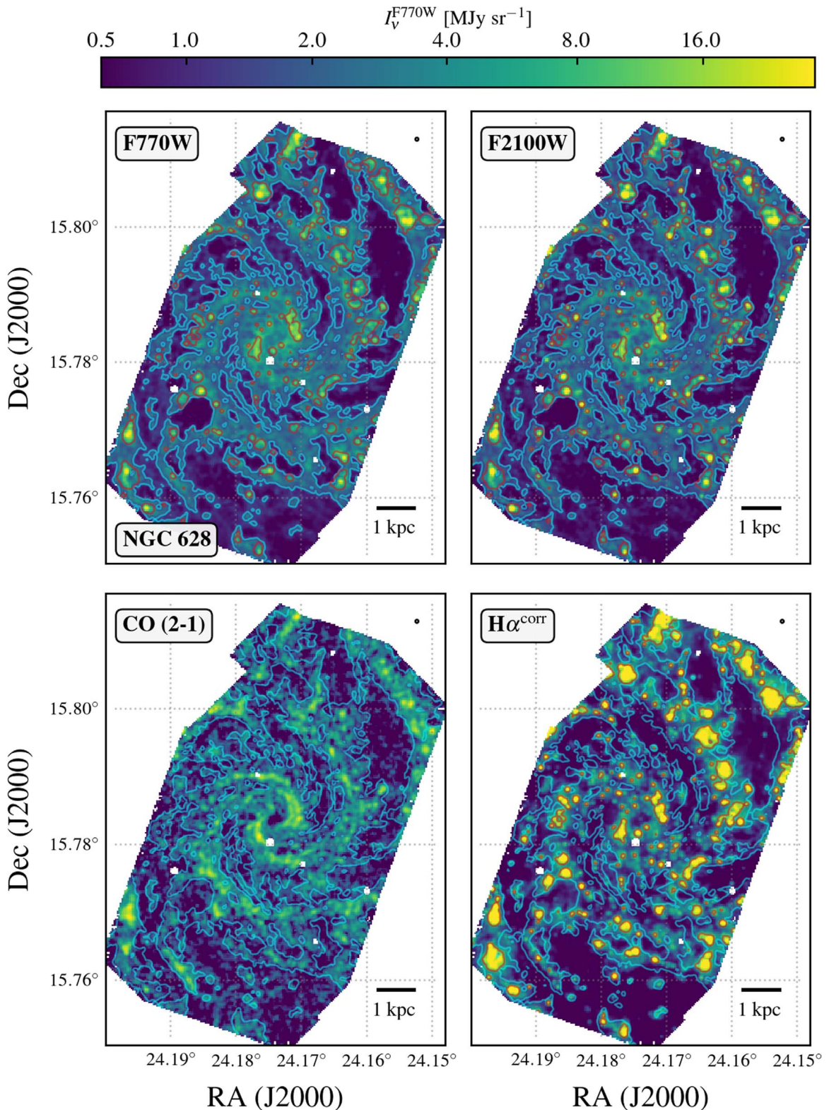
Figure 1. Mid-IR, CO, and extinction-corrected H \alpha maps for NGC 628. These images show our matched 80 pc resolution, matched astrometry data for NGC 628. The top row shows two of the four analyzed JWST mid-IR images, F770W and F2100W. The bottom row shows the ALMA CO (2–1) image and the VLT/MUSE extinction-corrected H \alpha . All images are displayed using an identical arcsinh stretch from 0.5 to 30 MJy sr ^{-1} after converting all bands to equivalent F770W using the band ratios in Table 1 for the mid-IR and the median ratios in Table 4 for CO (2–1) and H \alpha^{CORR} . We have blanked data outside the common JWST MIRI/MUSE/ALMA footprint. A scale bar shows 1 kpc at the distance of the galaxy and the 1'' (FWHM) beam appears in the top-right corner of the image. The blue contour in all panels shows an F770W contour at 1.5 MJy sr ^{-1} , and the red contour shows an H \alpha contour at an equivalent of F770W intensity 10 MJy sr ^{-1} .
