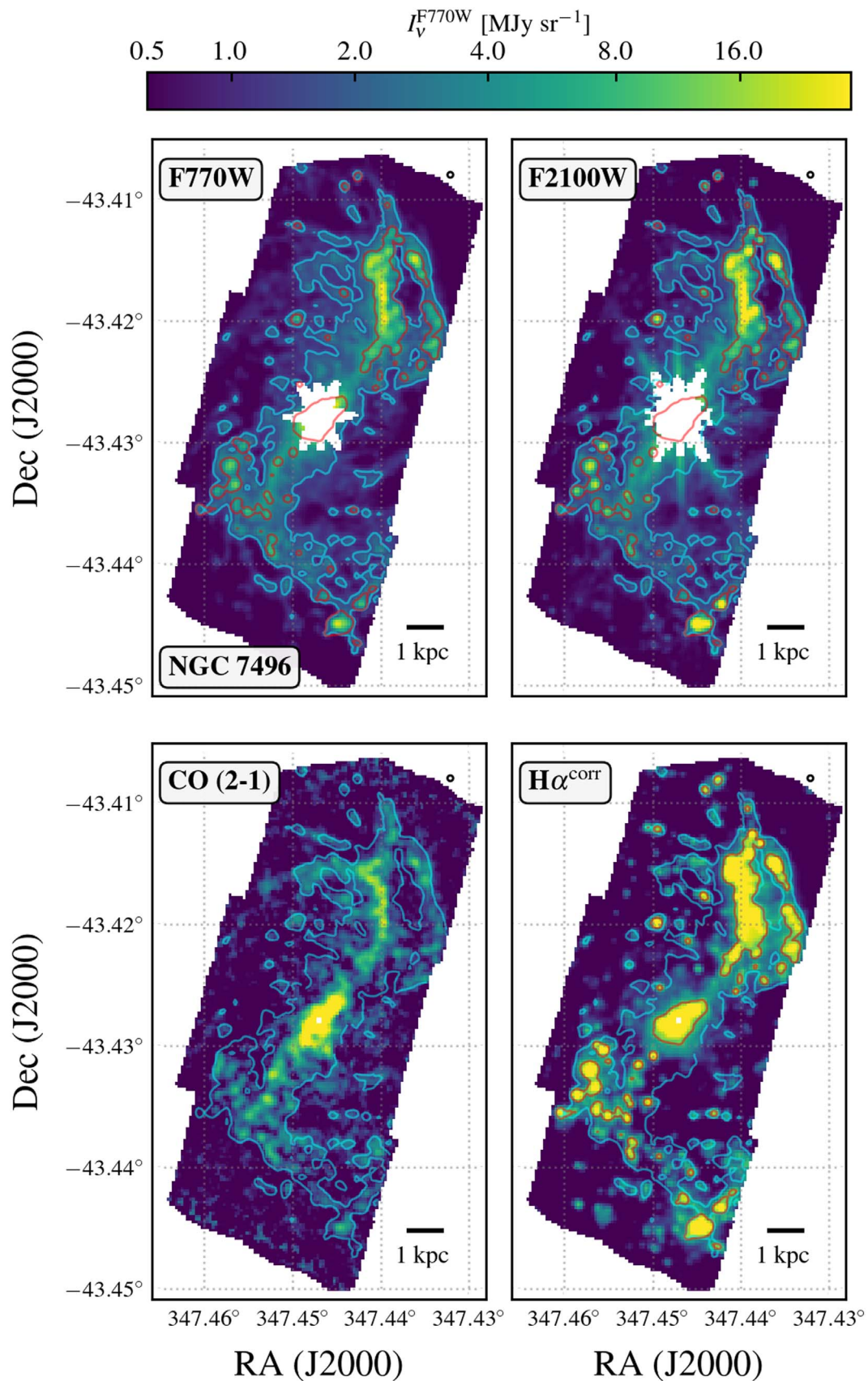
Figure 3. Mid-IR, CO, and extinction-corrected \text{H}\alpha maps for NGC 7496. As Figure 1 but for NGC 7496 at 150 pc resolution. As in that figure, the arcsinh stretch runs from 0.5 to 30 \text{MJy sr}^{-1} , and all bands are expressed in equivalent F770W intensity. As there, the blue shows an F770W contour at 1.5 \text{MJy sr}^{-1} , and the red shows an \text{H}\alpha contour at equivalent to 10 \text{MJy sr}^{-1} . Note the region blanked due to PSF effects at the galaxy center.
