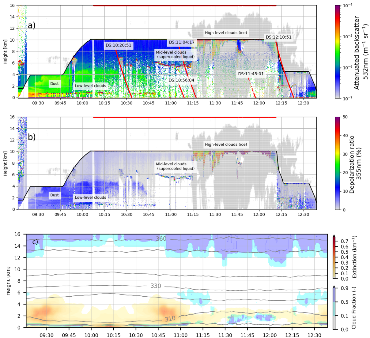
Figure 6. LNG-derived (a) backscatter signal at 532 nm and (b) depolarization ratio during the Safire FA20 flight 7 on 11 September 2021. Radar reflectivity is overlain in light gray. The reddish colors in (a) indicate clouds while the dust layer sampled at the beginning of the flight (between 0900 and 1045 UTC) between 1 and 5 km asl appears in green in (a) and blue in (b). (c) Vertical cross-section of dust extinction (warm colors), cloud water content (cold colors) and potential temperature along the Safire FA20 flight track extracted from the Meso-NH 4-km domain between 0900 and 1300 UTC.
