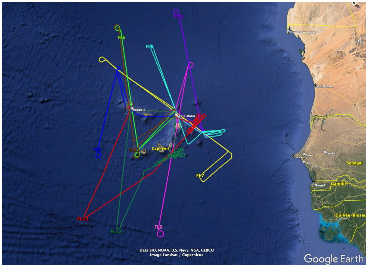
Figure 1. Safire FA20 flight tracks for the 9 flights conducted during the CADDIWA detachment in Cape Verde. Flights F5, F6, F9, F10 and F11 were made along Aeolus orbits. Flight F5 and F9 were conducted along morning orbits on 8 and 14 September, respectively. Flights F6, F10 and F11 were conducted along afternoon orbits on 10, 16 and 17 September, respectively. Flights F7 and F8 were made in the environment of tropical perturbation Pierre Henri on 11 September, and flights F12 and F13 in the environment of TS Rose on 18 and 19 September 2021. Map credit: © Google Earth 2021.
