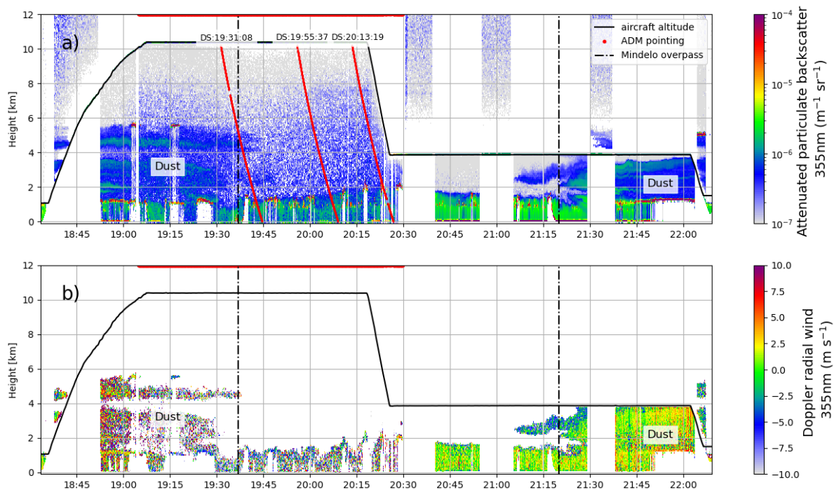
Figure 10. LNG-derived (a) backscatter signal at 355 nm and (b) Doppler radial wind during Safire FA20 flight 11 on 17 September 2021. The reddish colors in (a) indicate clouds. The dust layer sampled between 1830 and 1945 UTC and between 2100 and 2200 UTC above the boundary layer appears in blue in (a). The dash-dotted lines indicate the two overpasses of Mindelo on São Vicente Island. The flight track is shown in Figure 1 (brown track, tagged F11). The Safire FA20 was heading north during first overpass of Mindelo and heading south during the second overpass.
