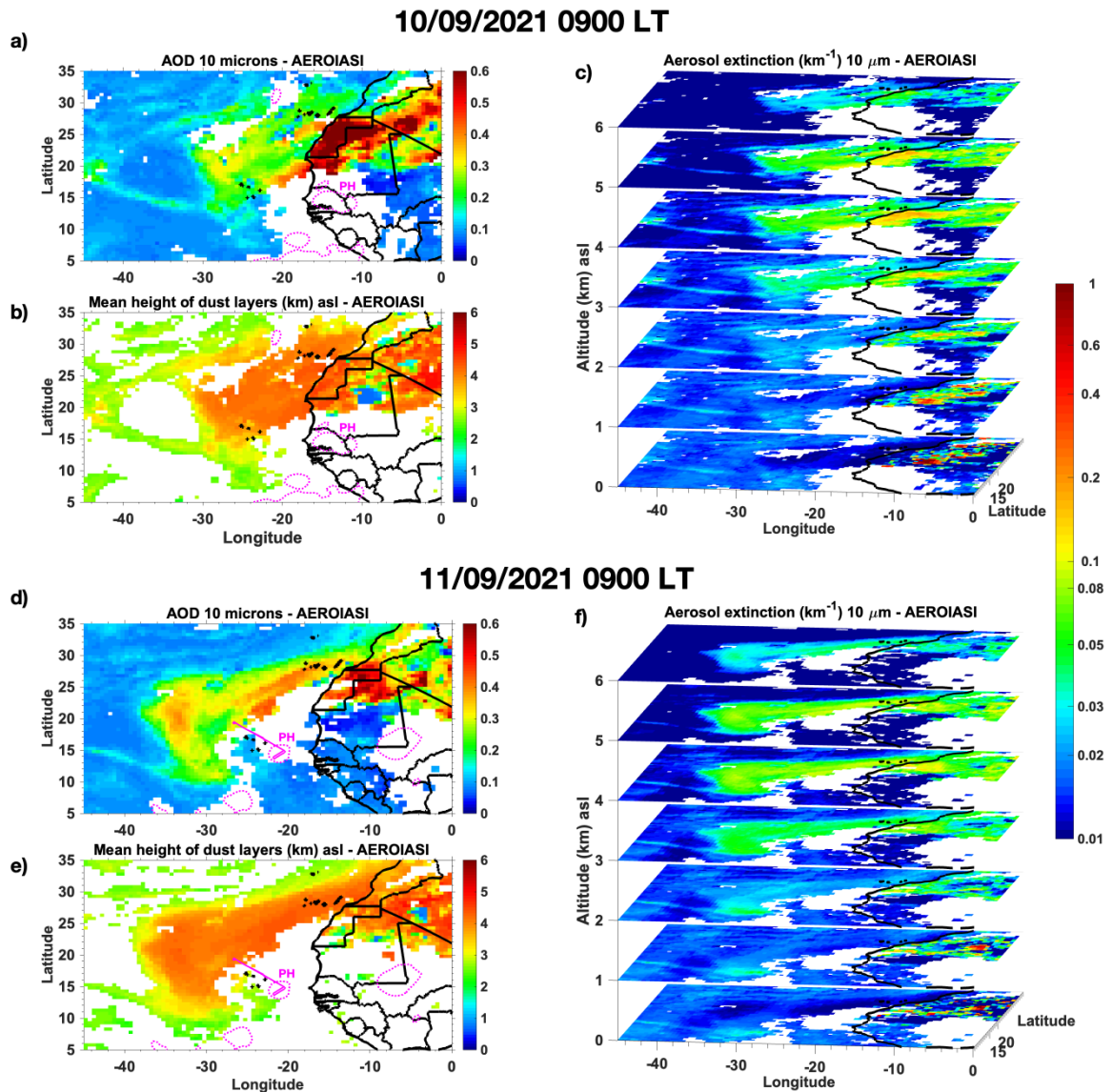
Figure 4. AEROIASI-derived dust AOD at 10\ \mu\text{m} (a), mean layer height (b) and 3D dust distribution (c) in the morning of 10 September 2021. These AEROIASI products are based on the IASI observations made from 3 platforms (MetOp A, B and C) merged together, the equatorial crossing time of which are separated by less than 1h, around 0900 LT Cape Verde (1000 UTC). Areas in white in the plots indicate the presence of clouds that prevent AEROIASI retrievals. The mean aerosol layer height is estimated as the height below which the AOD is half that of the total column. (d), (e) and (f) are the same as (a), (b) and (c), respectively but for 11 September in the morning. The magenta line in panels (d) and (e) is the Safire FA20 flight track. The dotted magenta contours represent brightness temperature isotherm 245 K indicative of the most active convective clouds associated with PH. The colorbar of the 3D plots in panels (c) and (f) is the one located on the rightmost part of the figure.
