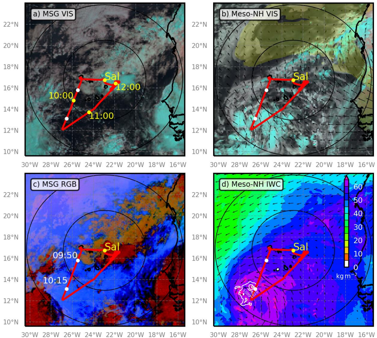
Figure 8. Weather situation on 19 September 2021 at 1000 UTC associated with the tropical disturbance that will become TS Rose later on that day. (a) MSG reflectance in the visible. (b) Synthetic reflectance in the visible from the Meso-NH model forecast and aerosol optical thickness ( > 0.1 ) in brown. Winds at 4 km altitude are also indicated (arrows). (c) RGB MSG image showing high clouds (red), mid-level clouds (dark brown) and low clouds (light brown), and terrigenous aerosols (pink). (d) TCWV in color, sea level pressure (white contour) and wind at 10 m (arrows). The Safire FA20 flight track is shown in red throughout the figures, the white dots locate the sondes dropped from the aircraft, and the black dot indicates the airport on Sal.
