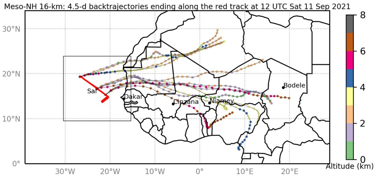
Figure 7. Meso-NH simulation on the 16-km resolution domain showing 4.5-day back trajectories ending at 1200 UTC and ending at 2.4, 2.7, 3.2 and 5.7 km asl along the Safire FA20 flight track shown in Figure 6c. Dots represent the evolution of the back trajectories every 3 h.
