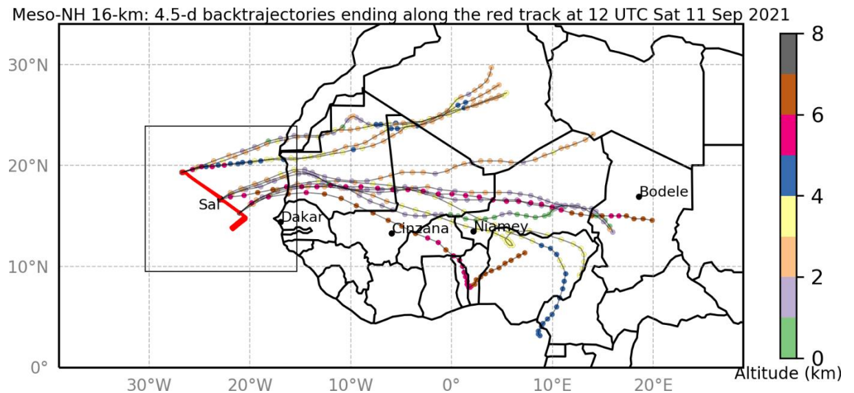
Figure 7. Meso-NH simulation on the 16-km resolution domain showing 4.5-day back trajectories ending at 1200 UTC and ending at 2.4, 2.7, 3.2 and 5.7 km asl along the Safire FA20 flight track shown in Figure 6c. Dots represent the evolution of the back trajectories every 3 h.
