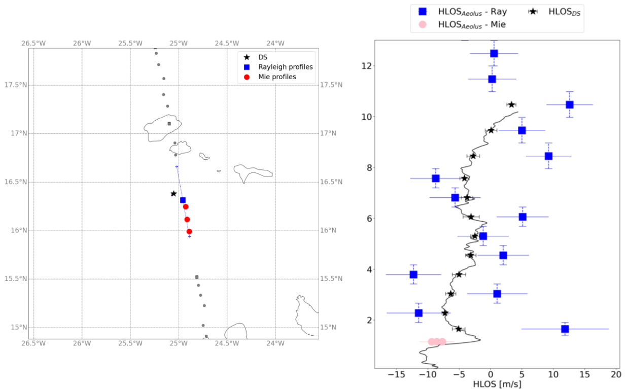
Figure 11. Left: Aeolus orbit (grey squares and grey circles, indicating the location of Aeolus L2B Mie and Rayleigh profiles, respectively) over Cape Verde on 17 September 2021 at 1936 UTC. The blue square corresponds to the location of the Aeolus L2B Rayleigh wind products used for comparison with the dropsonde (black star) released south of São Vicente at the time of the Aeolus overpass of the Safire FA20. The red filled circles correspond to the location of the Aeolus L2B Mie wind products used for comparison with the dropsonde. Right: Comparison between the dropsonde-derived HLOS velocity (black symbols) and Aeolus-derived Mie HLOS velocity (red circles) and Rayleigh HLOS velocity (blue squares). The dropsonde was released at 1931 UTC. Error bars associated with the Aeolus product are also shown as colored horizontal lines.
