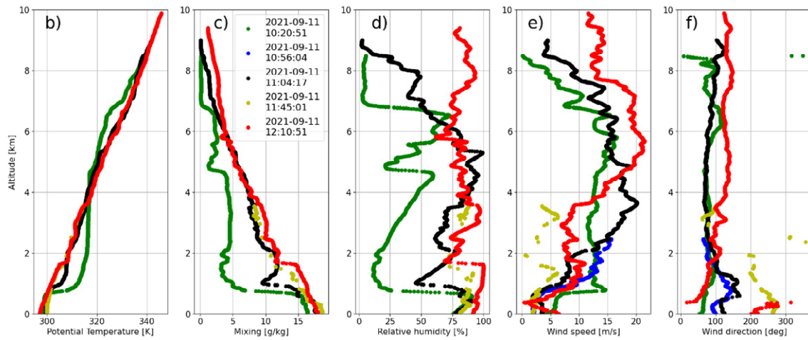
Figure 5. (a) Safire FA20 flight track (red) overlain on the Spinning Enhanced Visible and Infrared Imager (SEVIRI) dust RGB composite at 1100 UTC on 11 September. Pink indicates the presence of dust while dark red indicates high-level clouds. The location of the dropsonde releases are also shown as white dots. The Cape Verde Islands are highlighted by thick black lines. The two black circles indicate the distance from Sal, the outer one being at 425 NM and the inner one at 225 NM. Bottom: Profiles of potential temperature (b), water vapor mixing ratio (c), relative humidity (d), wind speed and direction (e, f) obtained from the five dropsondes released from the Safire FA20 in the morning of 11 September 2021 (DS1 in green, DS2 in light blue, DS3 in yellow, DS4 in grey and DS5 in dark blue).
