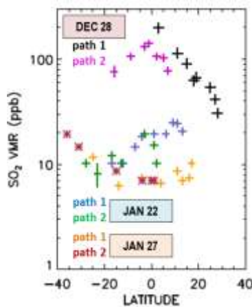
Fig. 2 \text{SO}_2 gas abundance retrieved from the 2010/2011 HST data; two paths or maps were observed on each date as indicated by the color legend
