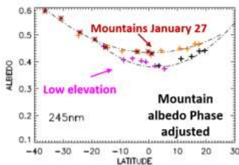
Fig. 4 Smooth increases in the cloud top 245 nm albedo with increasing latitude were observed over the plains and over Aphrodite Terra. The 20^\circ higher phase angle value associated with the December 2010 observations produces a \sim 20\% brightening in the cloud top albedo in December 2010 relative to the January 2011 dates. Therefore, to make a legitimate comparison of the albedo levels between the two terrain types we apply this brightening scale factor to the January albedo data.
