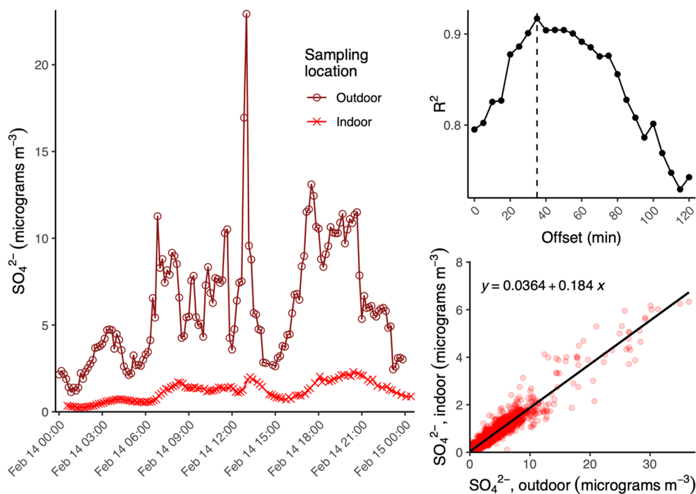
Figure 6. Indoor and outdoor PM sulfate as measured by the JHU HR-AMS at the house site. Date times are in AKST. The left panel shows the time series of sulfate, bottom right shows the correlation between indoor and outdoor PM sulfate, and the top-right shows the degree of correlation ( R^2 ) for a lagged correlation between indoor and outdoor PM sulfate observations.
