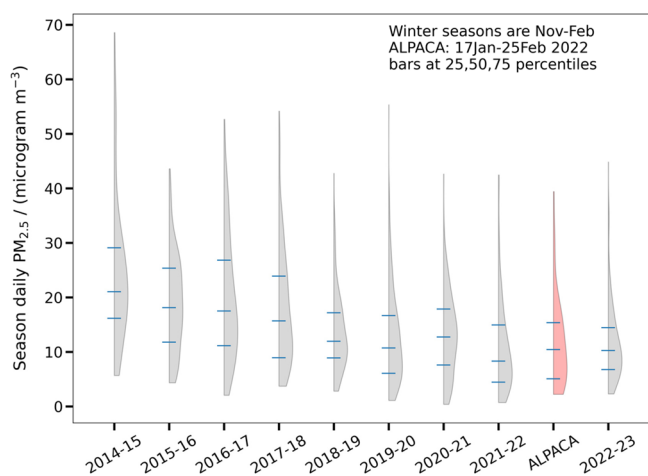
Figure 5. Probability density distributions of daily average particulate matter concentrations ( PM_{2.5} ) from NCore (ADEC/EPA measurements) during recent winters (November of the first year to end of February of the second year listed). The red figure shows the distribution during the ALPACA field study, a subset of the 2021–2022 winter season's data. Bars within each distribution represent the first quartile, median, and third quartile of the distribution.
