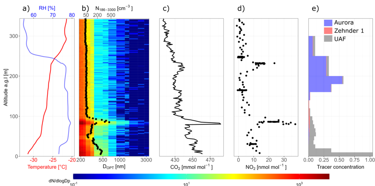
Figure 9. Helikite profile of the vertical structure of the atmosphere from 09:50 to 10:35 AKST on January 30, 2022. (a–d) Temperature, RH, particle counts, and CO 2 are part of the Helikite measurement payload, and NO 2 was measured with the LAERO-CNRS (CASPA) MicroMegas package. The right-most panel (e) shows power plant tracer forecasts for January 30, 2022 as a function of altitude at the UAF Farm site. On this day, tracers originating from the UAF and Aurora power plants, along with a small contribution from Zehnder power plant were forecast to arrive over the UAF Farm site. See text for details.
