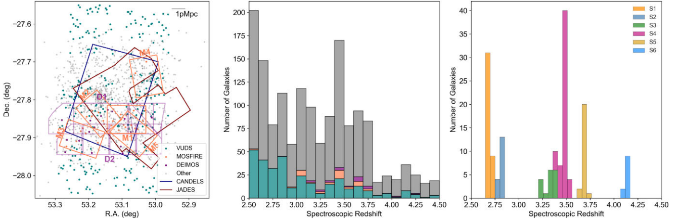
Figure 1. Left: The spatial distribution of galaxies with a secure spectroscopic redshift falling within the range of 2.5 < z < 4.5 . Galaxies are coloured based on the survey from which the spectroscopic redshift was obtained: the VUDES survey (green/blue), C3VO MOSFIRE (orange) and DEIMOS (purple), and a compilation of other spectral surveys (grey, see text). The footprints of the GOODS-S and JADES surveys are also shown. Centre: Stacked histogram representing the spectroscopic redshift distribution of all galaxies with a secure z_{\text{spec}} in this range adopting the same colour coding as in the left panel. Right: The redshift distribution of the spectroscopic members of each of the six different protostructures presented in this study as labeled in Fig. 2.
