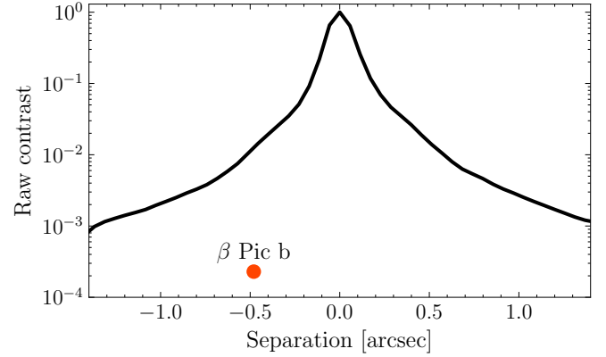
Fig. 2. Raw white light contrast curve for our CRiRES+ observations. The location of \beta Pictoris b is indicated in this diagram according to the K -band contrast from Chilcote et al. (2017).
