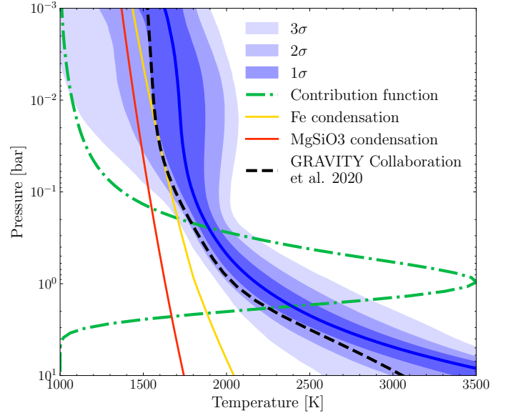
Fig. 5. Retrieved P - T profile for the nominal model with associated uncertainties. Also shown: the P - T profile obtained by GRAVITY Collaboration (2020), the condensation curves of Fe and MgSiO 3 for the best fitting parameters, and the emission contribution function for the best fitting parameters.
