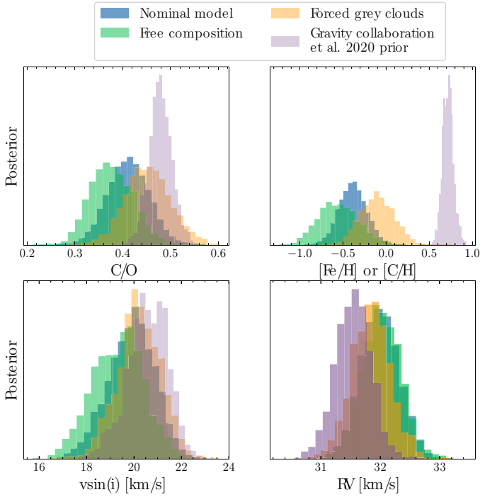
Fig. 4. Constraints on a subset of the parameters from the atmospheric retrievals using the models discussed in Sect. 4. The RV shown here is in the barycentric restframe.
