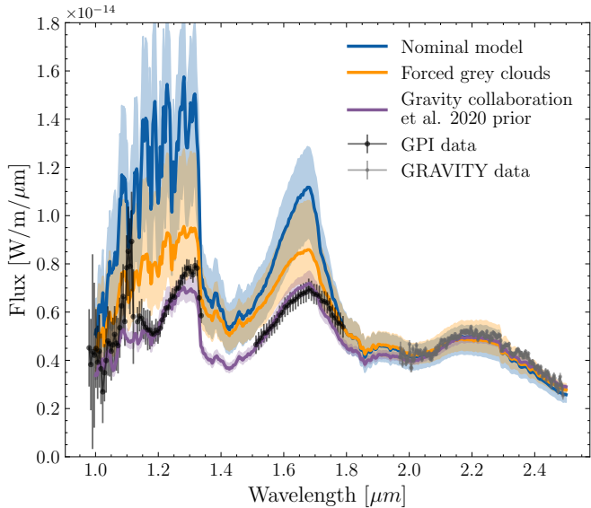
Fig. 7. Comparison of the spectral energy distributions of our retrieved models compared to the low-resolution GPI data from Chilcote et al. (2017) and GRAVITY data from GRAVITY Collaboration (2020). Since we do not retrieve radius, the flux of our models is scaled such that it matches the GPI flux in the K -band. The solid line shows the median value and the colored region shows the 16th and 84th percentiles.
