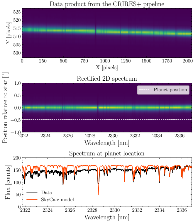
Fig. 1. Visualization of the data extraction pipeline. Top row shows the product of the obs_nodding recipe from the ESO CRiRES+ data reduction pipeline. The middle row shows the rectified 2D spectrum corrected for the slit tilt and curvature using pycrres and the bottom row shows the spectrum at the location of the planet, plotted together with a telluric model generated with SkyCalc.
