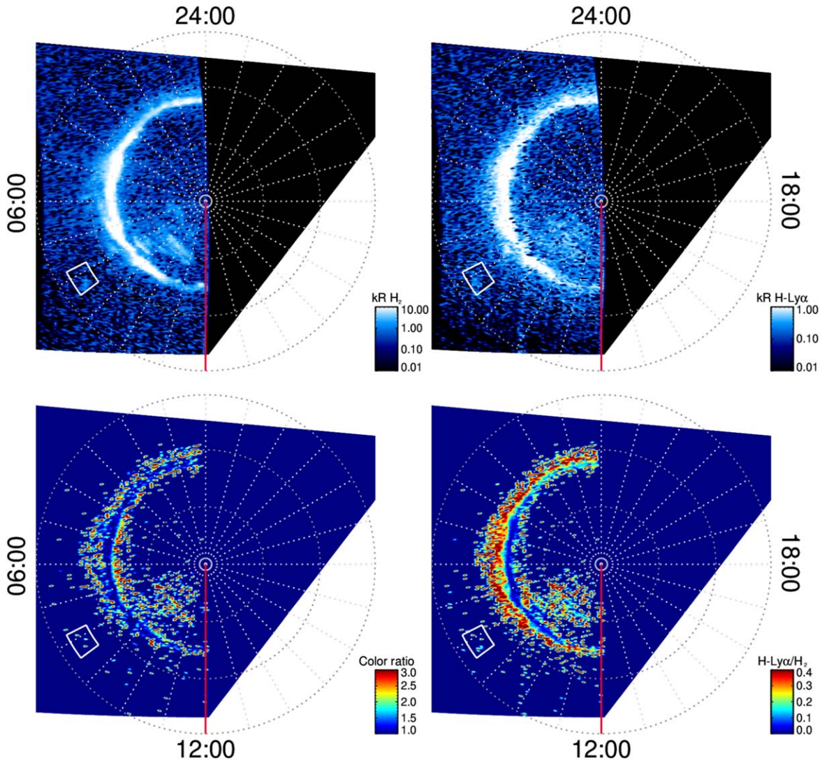
Figure 5. Polar projections of physical observables derived from the UVIS FUV processed observation of 2008 August 26 at 00:53:35. Top left: total H_2 brightness corrected for absorption. Top right: H Ly \alpha brightness corrected for absorption and underlying H_2 contribution. Bottom left: CR. Bottom right: H Ly \alpha / H_2 BR. Duplicated from Magalhães et al. (2019).
