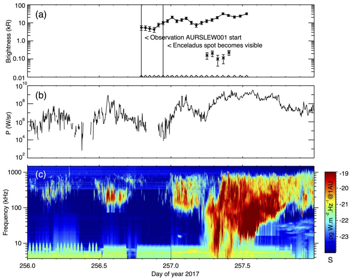
Figure 8. (a) The AURSLEW001 EUV image times are indicated by \wedge symbols. The vertical lines indicate when AURSLEW001 began and when the search box rotated into view and the Enceladus spot becomes visible, if present. The five actual spot detections are shown with the EUV brightnesses (in kR) and 1\sigma error bars indicated. The last three images did not have detections, possibly because the main auroral oval had expanded and brightened, increasing the background. Also shown (filled circles) are the peak brightness values in each image due to the main aurora with 5\sigma error bars. (b) The corresponding SKR power is shown from the Cassini RPWS. (c) The corresponding SKR spectrum is shown from the Cassini RPWS.
