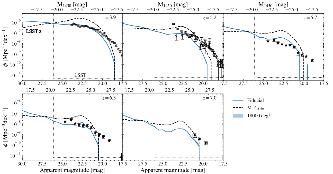
Figure 14. Same as for Fig. 12, but in the LSST z band. Blue shaded regions show the total field-to-field variance of the LF when assuming the LSST survey area ( 18000 \text{ deg}^2 ), although the region is almost invisible due to the small variance. The variance for 18000 \text{ deg}^2 is estimated by extrapolating from those up to 40 \text{ deg}^2 . The dotted lines correspond to the magnitude limit and survey area of the LSST survey ( 26.1 \text{ mag} in the z band, 18000 \text{ deg}^2 ).
