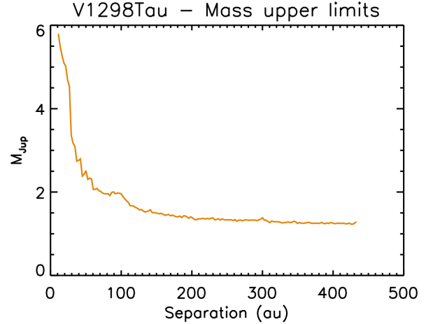
Fig. 9. Mass detection limits ( 5\sigma ) obtained from the SPHERE data (both IRDIS and IFS) expressed in units of Jovian mass as a function of the separation expressed in astronomical units.
