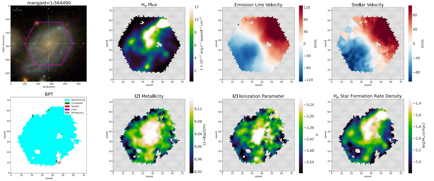
Figure 5. The physical properties of the SDSS MaNGA galaxy 1-564490. The top panels show from left to right the SDSS three-color image, the H\alpha line emission map, the H\alpha line velocity map, and the stellar velocity map. The bottom panels shows the BPT diagram and maps of IZI metallicity, IZI ionization parameter, and the density of star formation rate (SFR).
