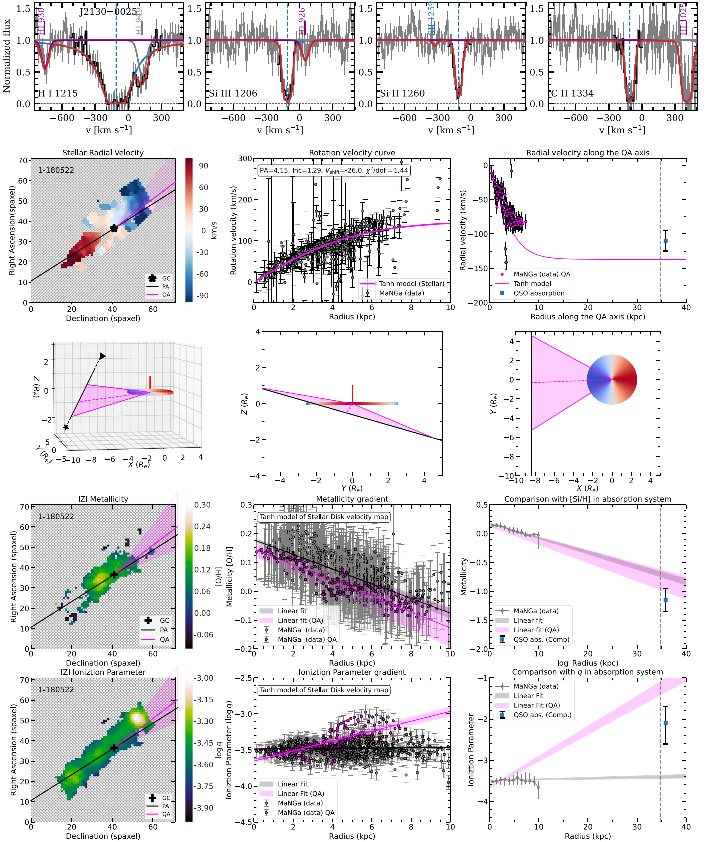
Figure 19. Comparison of radial velocity, metallicity, and ionization parameter derived from the fitting to MaNGA maps of the galaxy 1-180522 and those measured in the absorption system toward the quasar J2130–0025. A detailed description is presented in Appendix B.
