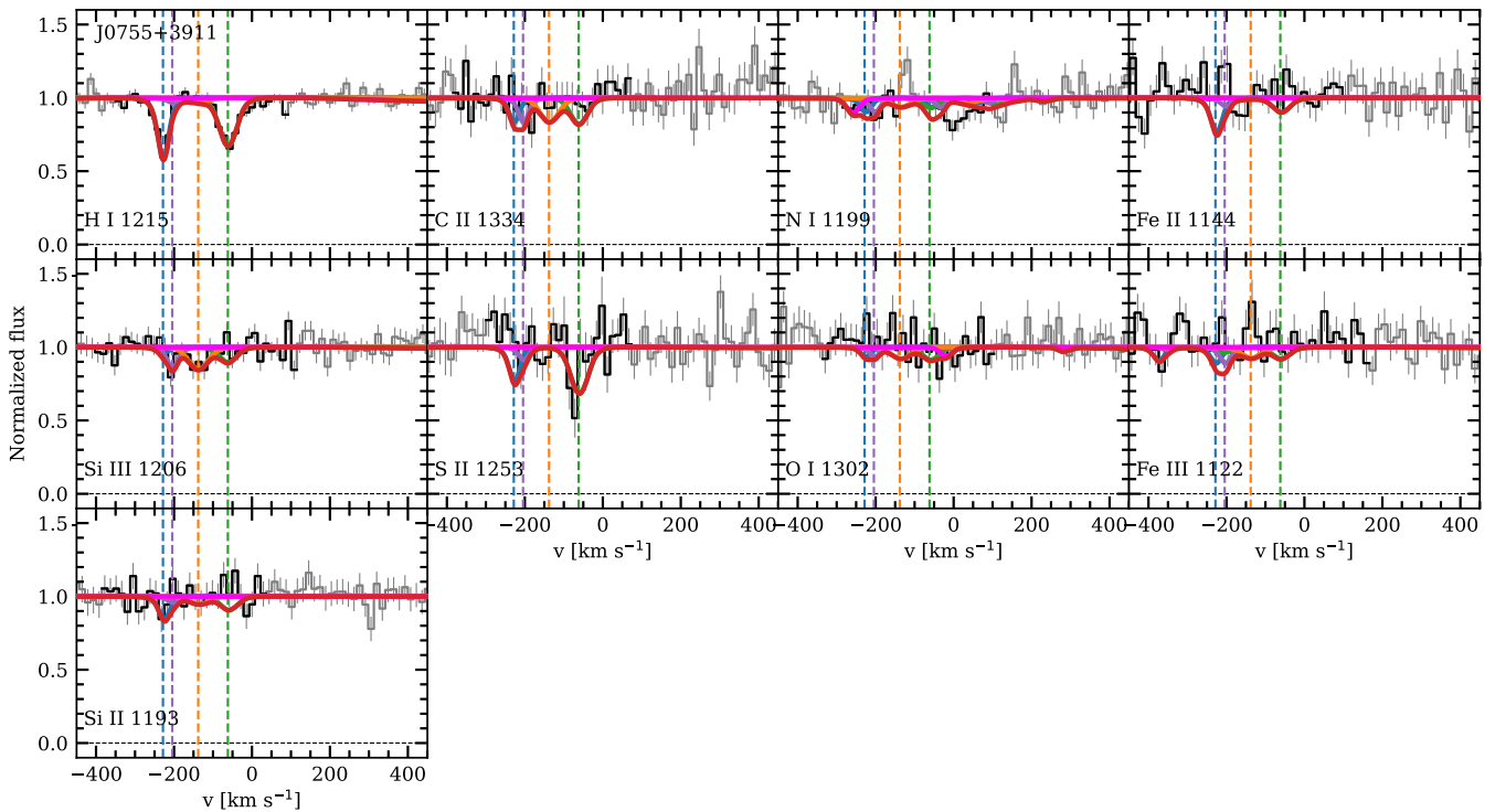
Figure 32. Fit to absorption lines at z_{\text{abs}} = 0.03362 in the spectrum of J0755+3911. Lines are the same as in Figure 27.
