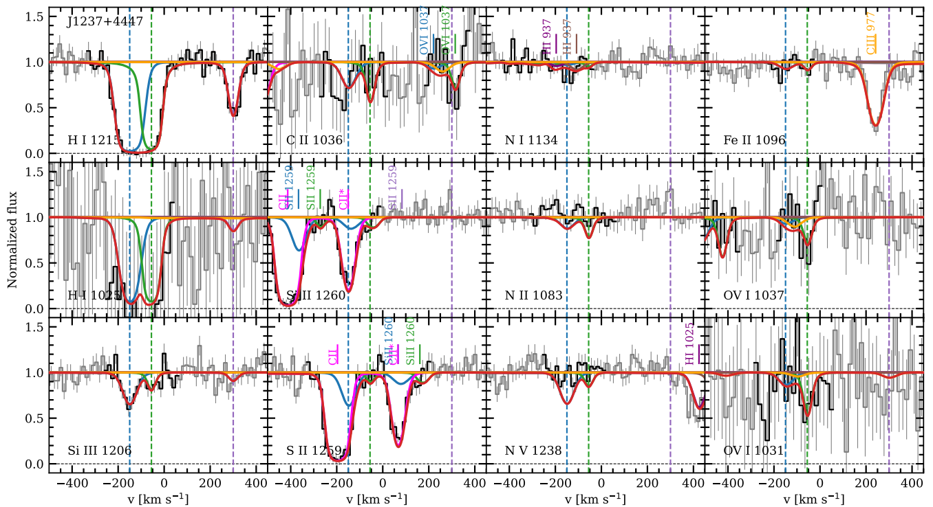
Figure 28. Fit to absorption lines at z_{\text{abs}} = 0.06013 in the spectrum of J1237+4447. Lines are the same as in Figure 27.
