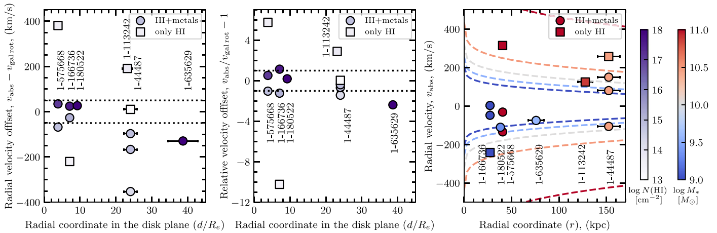
Figure 11. The left panel shows the difference between radial velocities of HI absorption components in quasar sight lines and predicted velocity of galaxy rotational models as a function of radial coordinate. Circles and squares represent components with both HI and metal lines and only HI, respectively. The color encodes the HI column density of the components. The horizontal dotted lines show the range of velocities from -50 to 50 \text{ km s}^{-1} . The middle panel is the same as the left panel, but shows the velocity offset in units of the predicted velocity of galaxy rotational models. Dotted lines represent the \pm 1 offsets relative to the predicted velocity (offset = 0). The right panel shows the radial velocity of absorption calculated in the galaxy rest frame as a function of the radial coordinate. The symbols are the same as in other panels. Color encodes the stellar mass of nearby galaxies. The curves show the escape velocity as a function of the distance for stellar masses of \log M_*/M_\odot = 9, 9.5, 10, 10.5, 11 . See the text for more details.
